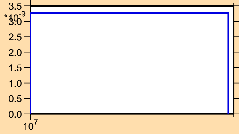
\sigma vs. E for ^{148}\text{Nd}(n,\text{nt})
