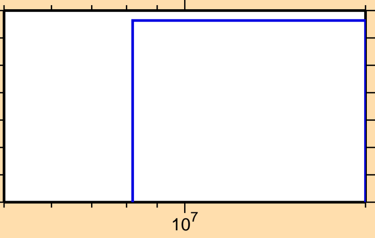
\sigma vs. E for ^{148}\text{Nd}(n,\text{nt})
