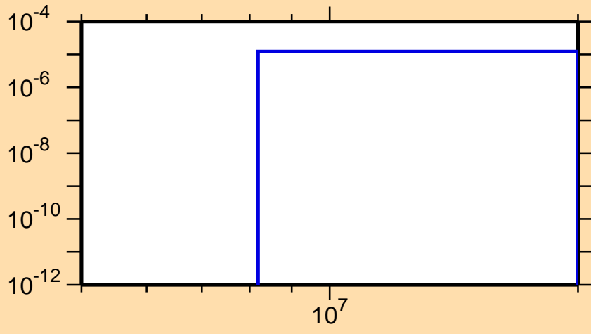
\sigma vs. E for ^{148}\text{Nd}(n,t)
