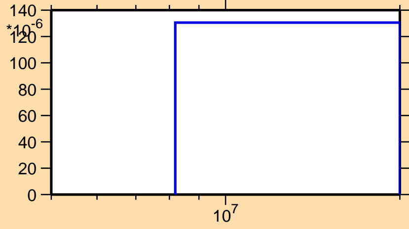
\sigma vs. E for ^{148}\text{Nd}(n,d)
