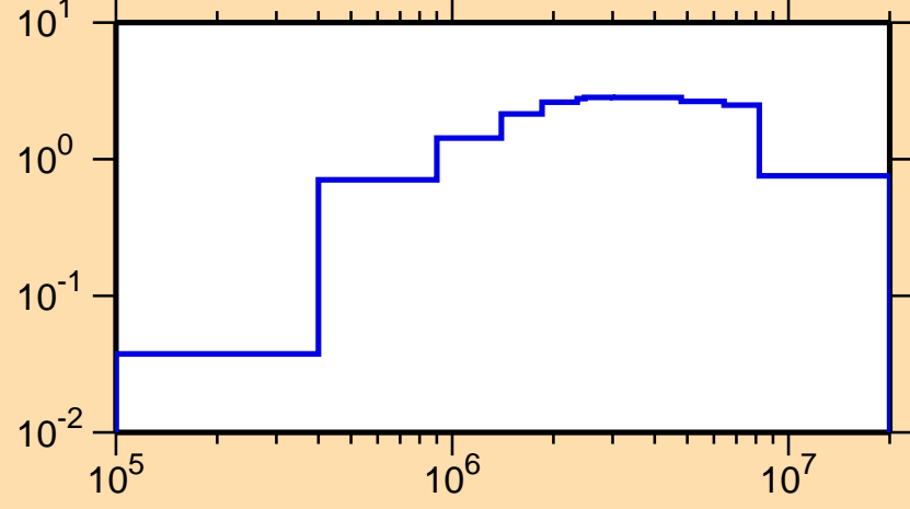
\sigma vs. E for ^{148}\text{Nd}(n,\text{inel.})
