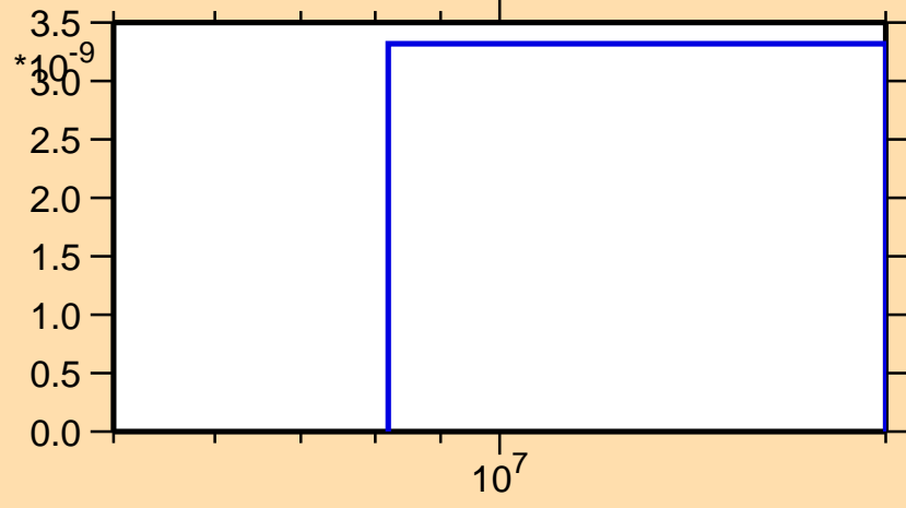
\sigma vs. E for ^{148}\text{Nd}(n,\text{nt})
