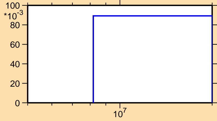
\sigma vs. E for ^{148}\text{Nd}(n,3n)
