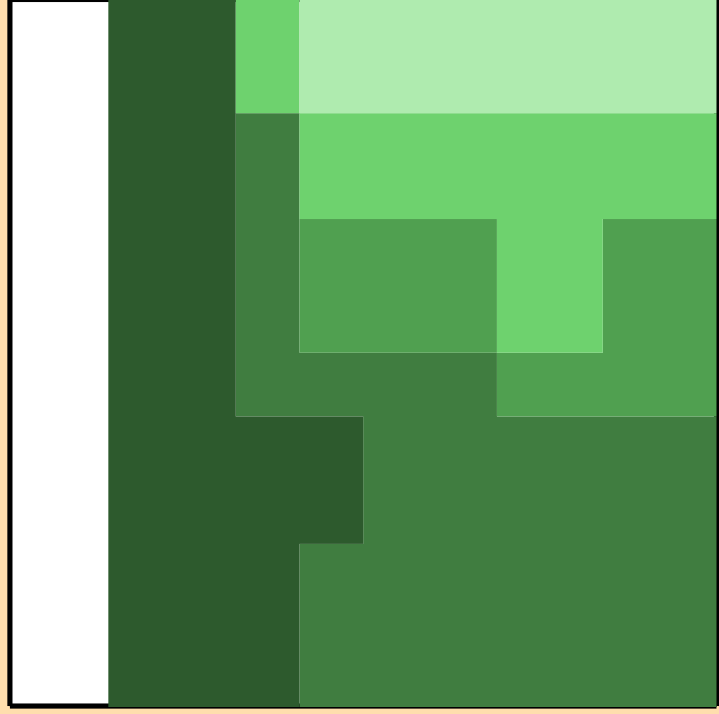
\Delta\sigma/\sigma vs. E for ^{150}\text{Nd}(n,p)
