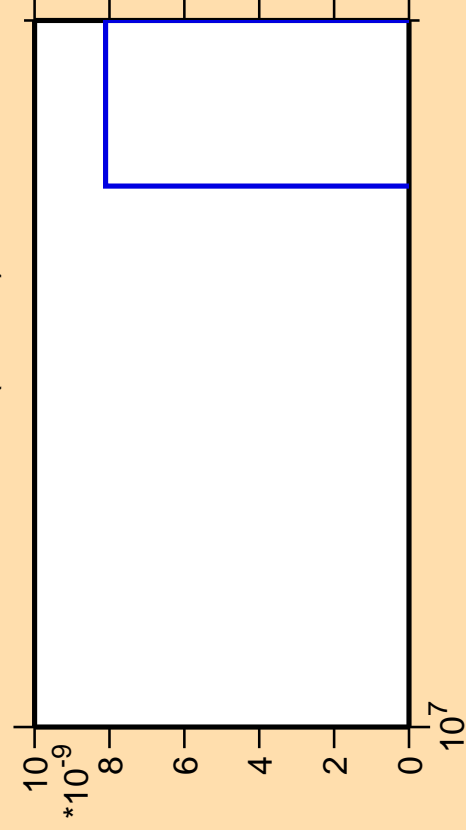
\Delta\sigma/\sigma vs. E for ^{150}\text{Nd} (mt 11)
