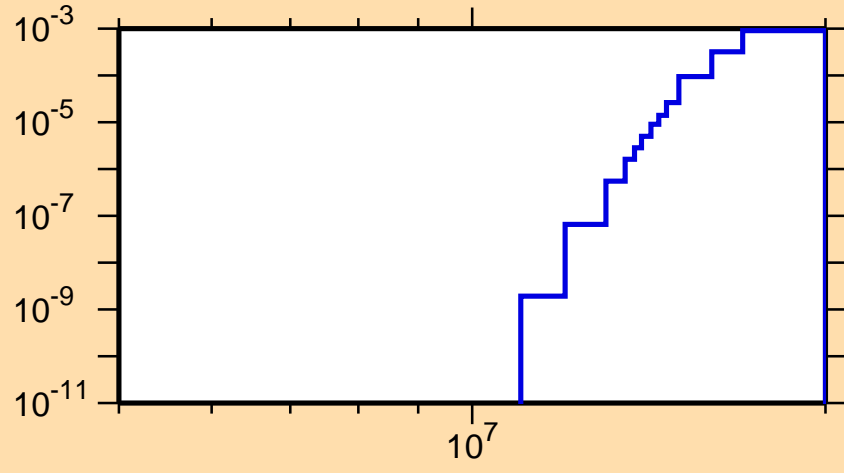
\sigma vs. E for ^{150}\text{Nd}(n,d)
