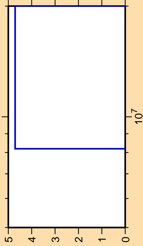
\Delta\sigma/\sigma vs. E for ^{150}\text{Nd}(n,2np)
