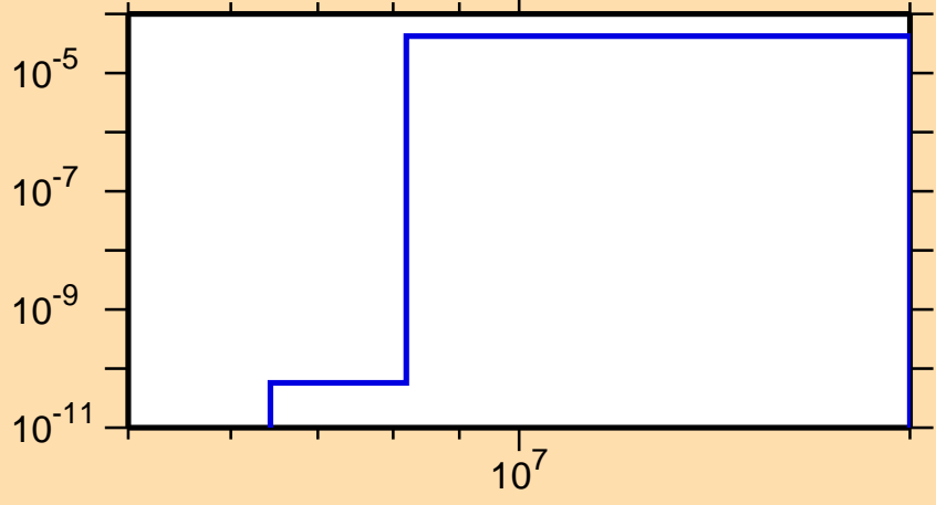
\sigma vs. E for ^{150}\text{Nd}(n,\alpha)
