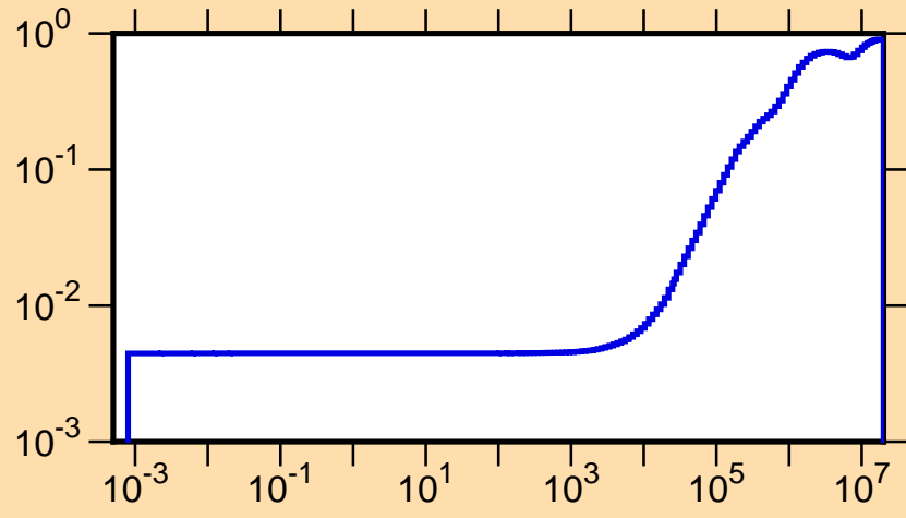
\mu vs. E for ^{151}\text{Nd}(\text{mt251})
