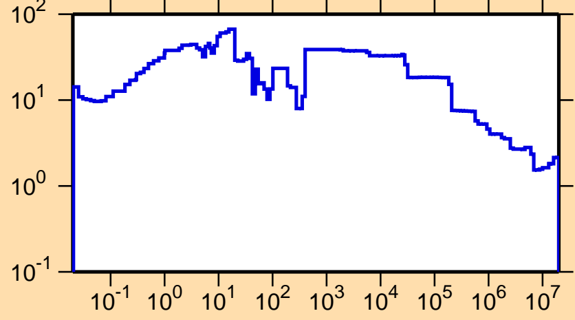
\Delta\sigma/\sigma vs. E for ^{151}\text{Nd}(n,\text{tot.})
