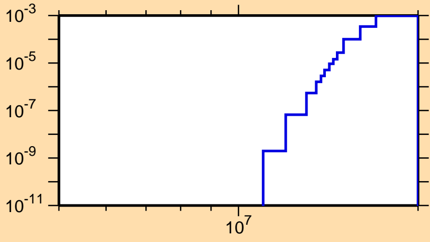
\sigma vs. E for ^{151}\text{Nd}(n,d)
