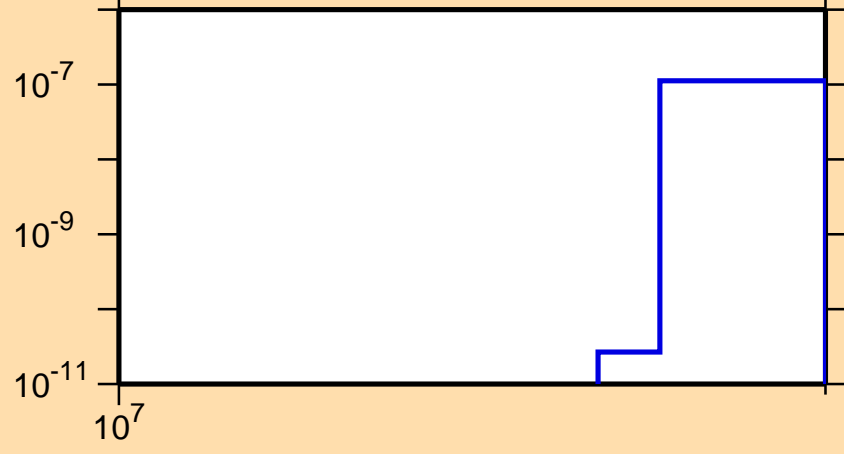
\sigma vs. E for ^{151}\text{Nd}(n,\text{nt})
