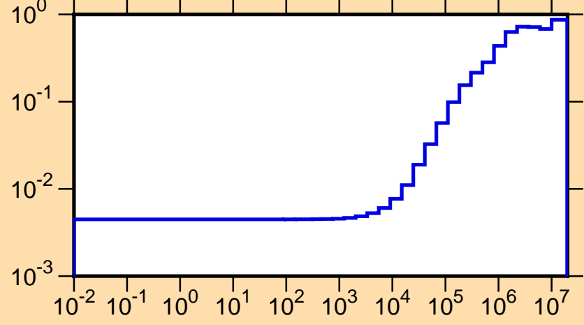
\mu vs. E for ^{151}\text{Nd}(\text{mt251})
