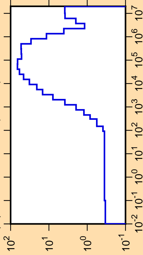
\Delta\mu/\mu vs. E for ^{151}\text{Nd}(\text{mt251})
