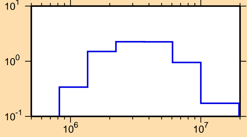
\sigma vs. E for ^{151}\text{Nd}(n,n\text{cont.})
