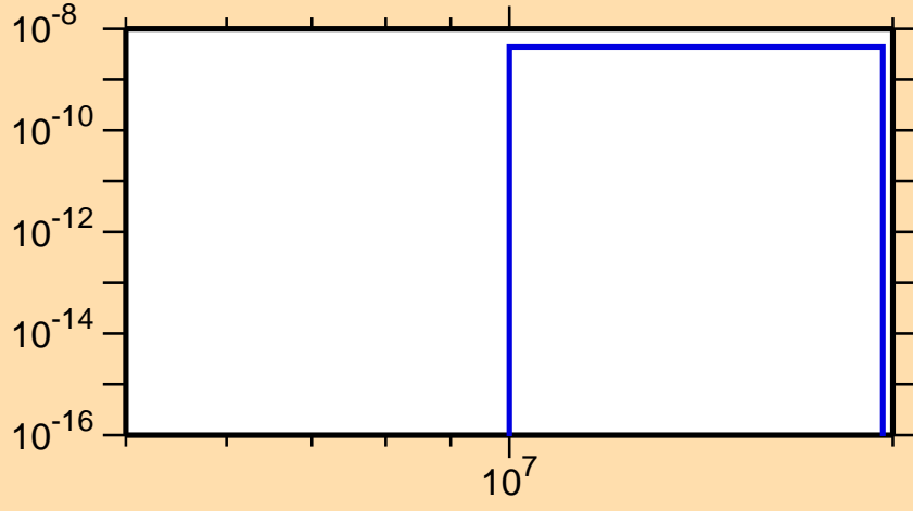
\sigma vs. E for ^{151}\text{Nd}(n,2n\alpha)
