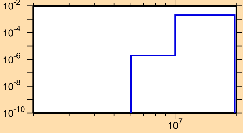
\sigma vs. E for ^{151}\text{Nd}(n,p)
