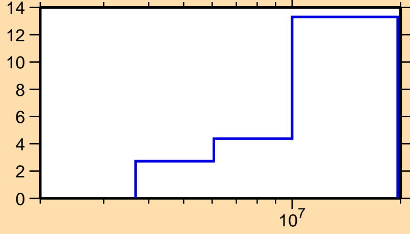
\Delta\sigma/\sigma vs. E for ^{151}\text{Nd}(n,ncont.)
