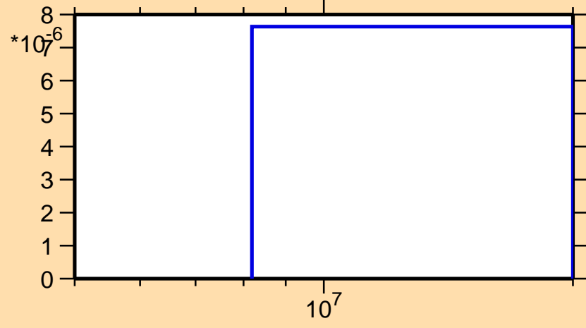
\sigma vs. E for ^{151}\text{Nd}(n,np)
