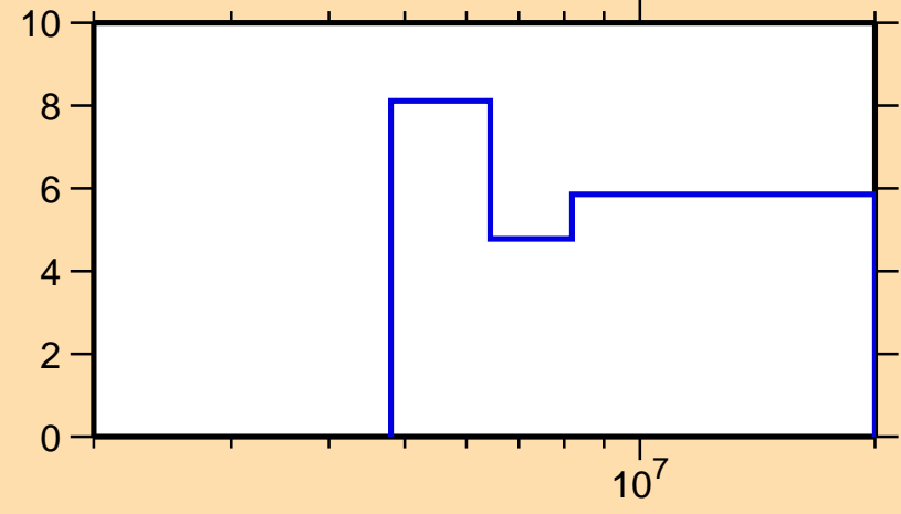
\Delta\sigma/\sigma vs. E for ^{151}\text{Nd}(n,2n)
