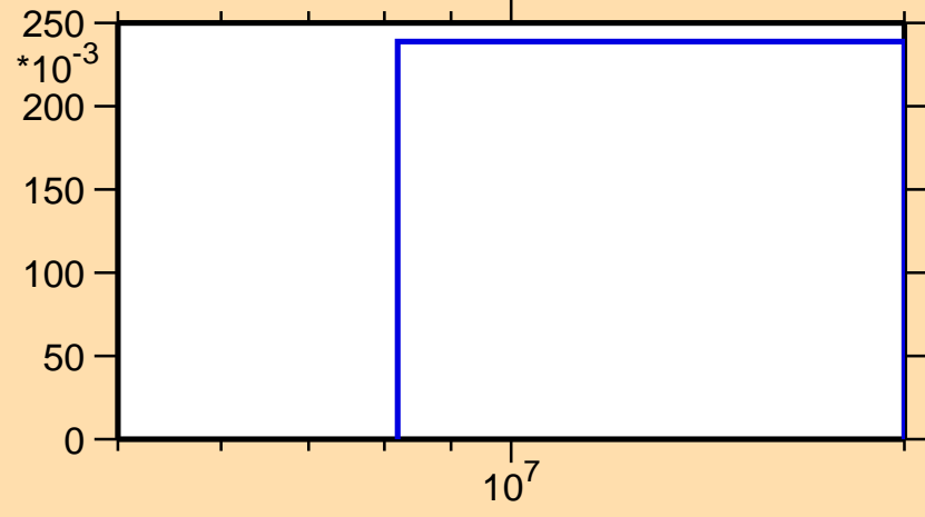
\sigma vs. E for ^{151}\text{Nd}(n,3n)
