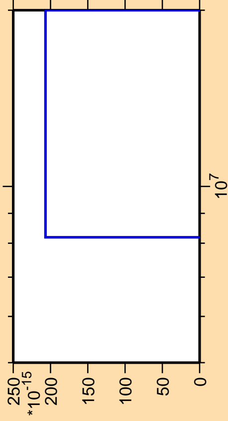
\Delta\sigma/\sigma vs. E for ^{151}\text{Nd}(\text{mt } 11)
