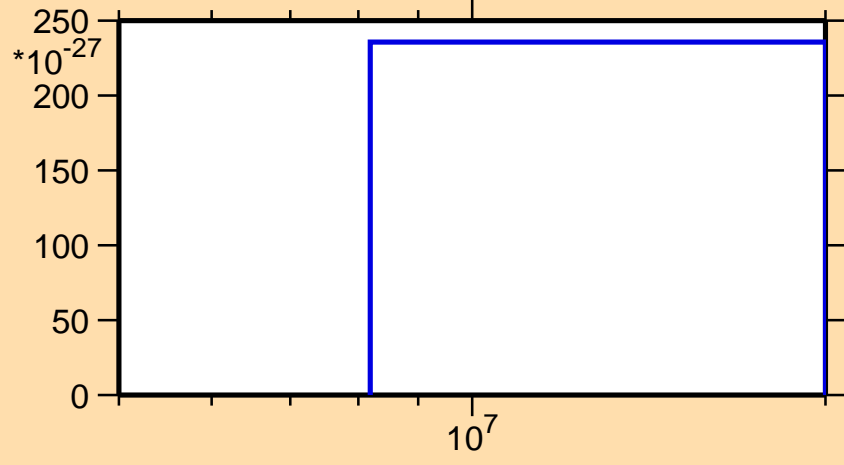
\sigma vs. E for ^{151}\text{Nd}(\text{mt } 11)
