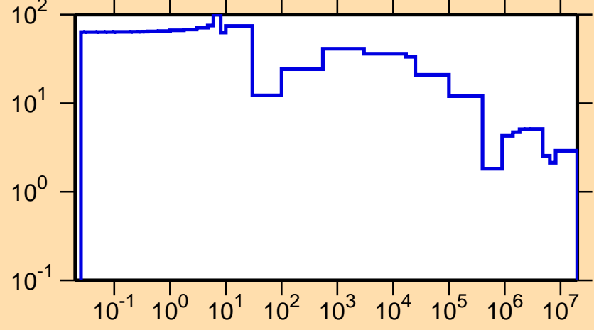
\Delta\sigma/\sigma vs. E for ^{151}\text{Nd}(n,\text{el.})
