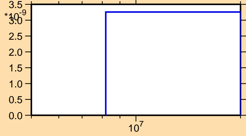
\sigma vs. E for ^{151}\text{Nd}(n,\text{nd})
