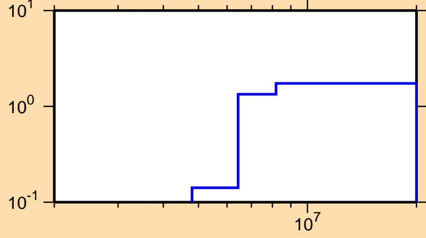
\sigma vs. E for ^{151}\text{Nd}(n,2n)
