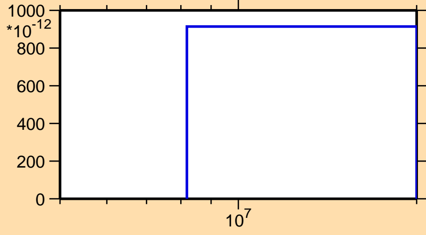
\sigma vs. E for ^{151}\text{Nd}(n,\text{nt})
