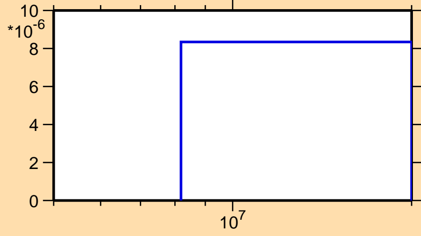
\sigma vs. E for ^{151}\text{Nd}(n,t)
