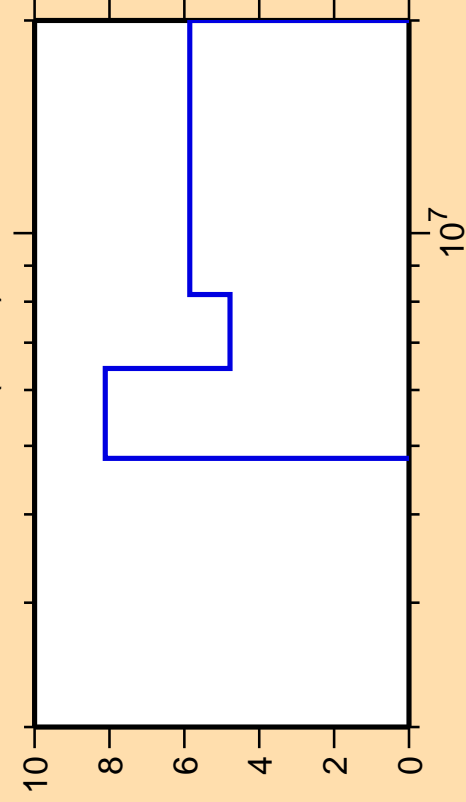
\Delta\sigma/\sigma vs. E for ^{151}\text{Nd}(n,2n)
