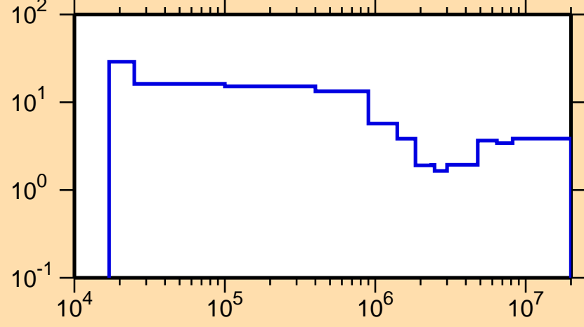
\Delta\sigma/\sigma vs. E for ^{151}\text{Nd}(n,\text{nonel.})
