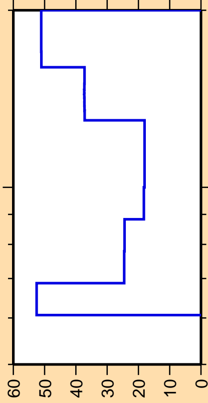
\Delta\sigma/\sigma vs. E for ^{154}\text{Nd}(n,2n)
