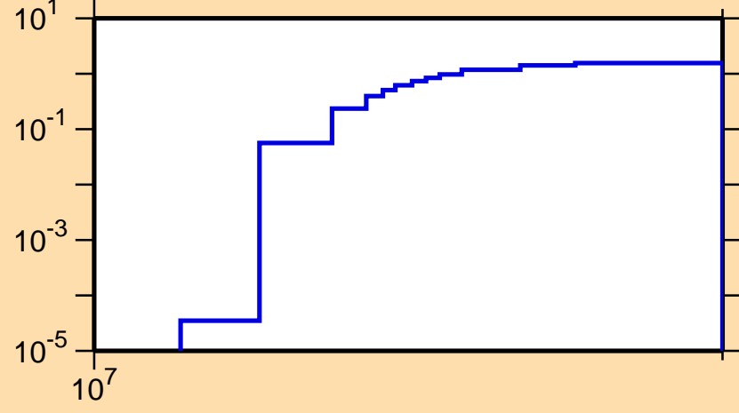
\sigma vs. E for ^{154}\text{Nd}(n,3n)
