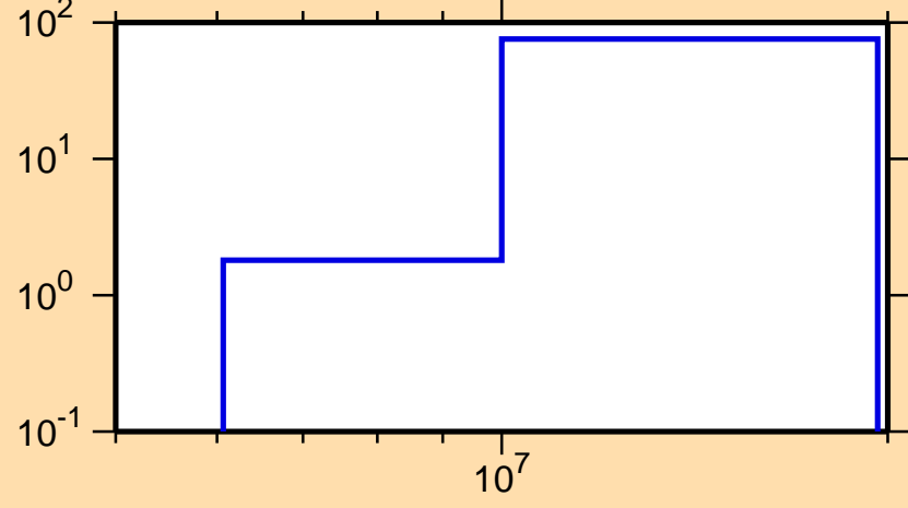
\Delta\sigma/\sigma vs. E for ^{154}\text{Nd}(n,p)
