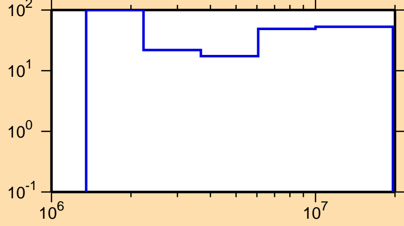
\Delta\sigma/\sigma vs. E for ^{154}\text{Nd}(n,n\text{cont.})
