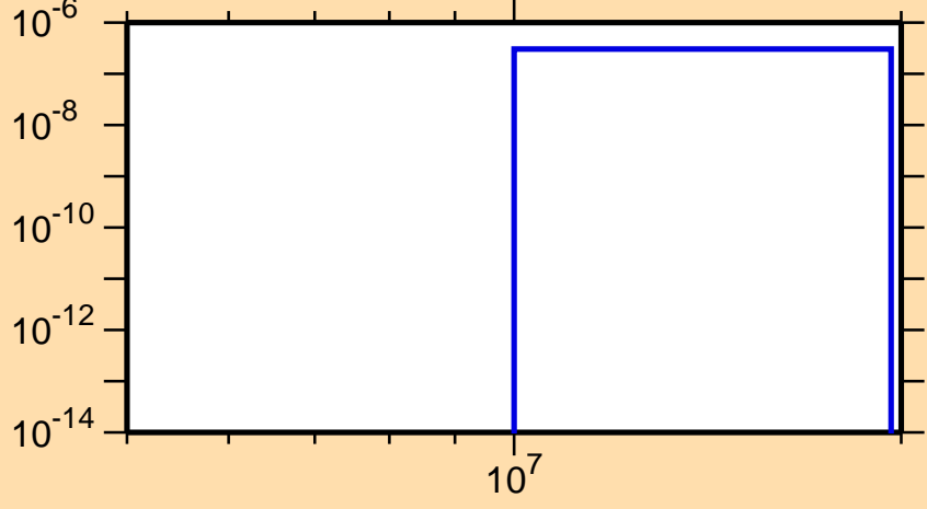
\sigma vs. E for ^{154}\text{Nd}(n,n\alpha)
