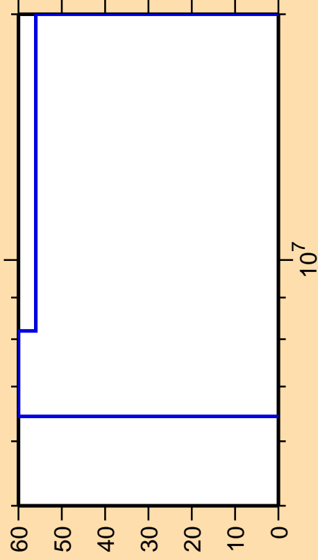
\Delta\sigma/\sigma vs. E for ^{154}\text{Nd}(n,\gamma)
