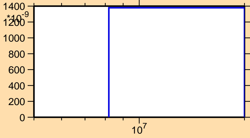
\sigma vs. E for ^{154}\text{Nd}(n,t)
