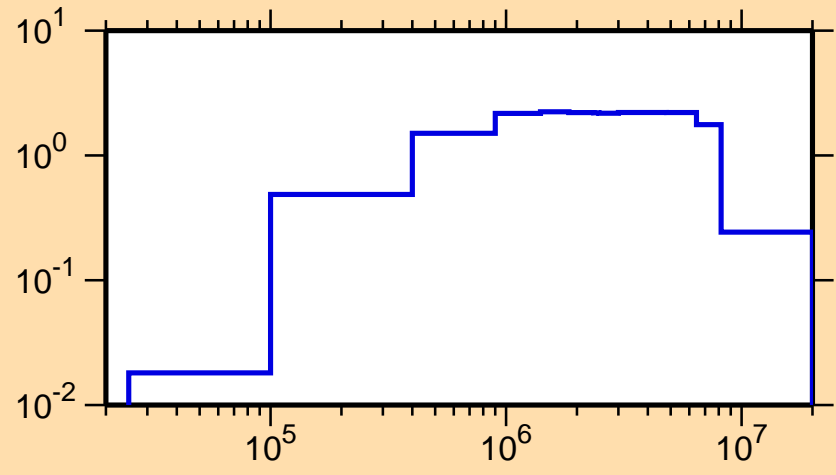
\sigma vs. E for ^{154}\text{Nd}(n,\text{inel.})
