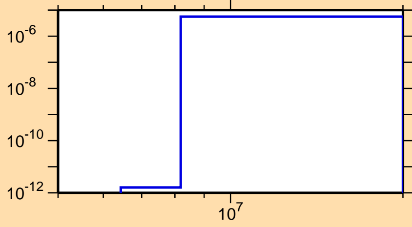
\sigma vs. E for ^{154}\text{Nd}(n,\alpha)
