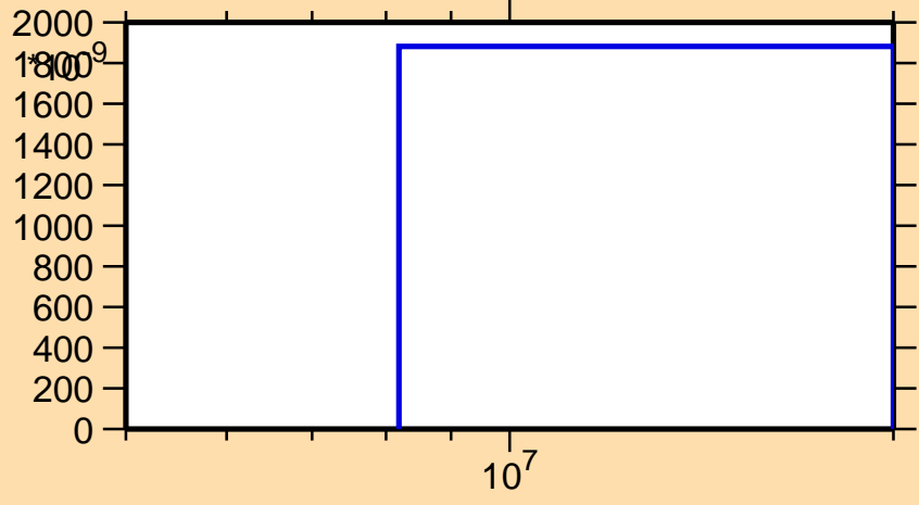
\sigma vs. E for ^{154}\text{Nd}(n,d)
