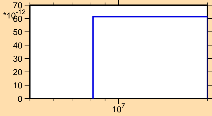
\sigma vs. E for ^{154}\text{Nd}(n,\text{nt})
