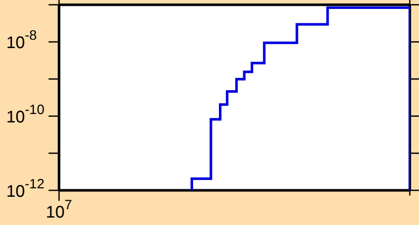
\sigma vs. E for ^{284}
