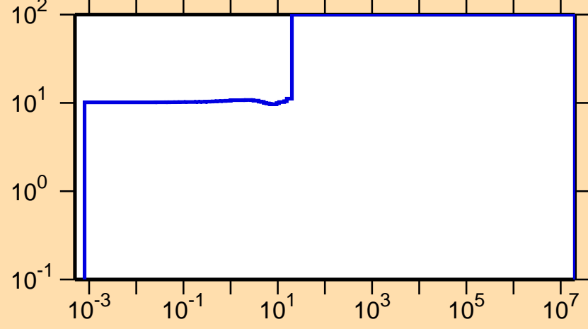
\Delta\sigma/\sigma vs. E for ^{285}\gamma
