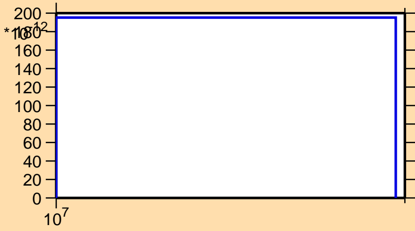
\sigma vs. E for ^{285}\alpha )
