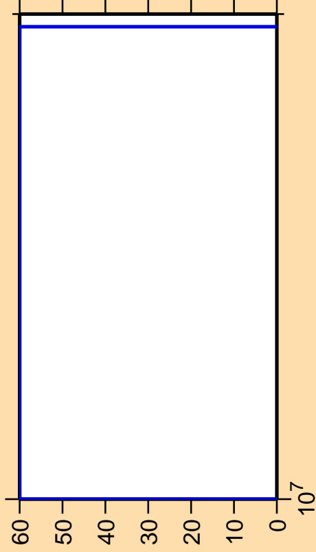
\Delta\sigma/\sigma vs. E for ^{285}\alpha )
