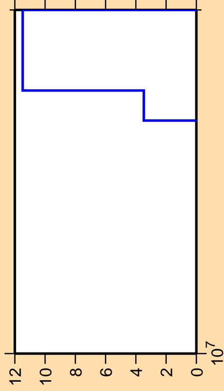
\Delta\sigma/\sigma vs. E for ^{287}\text{He3} )
