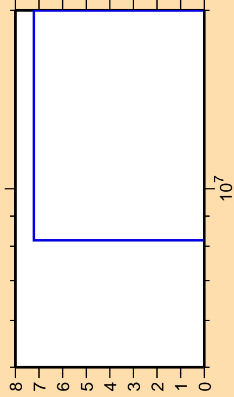
\Delta\sigma/\sigma vs. E for ^{287}
