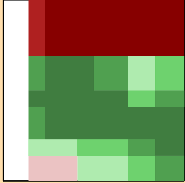
\Delta\sigma/\sigma vs. E for ^{251}\text{No}(n,2n)
