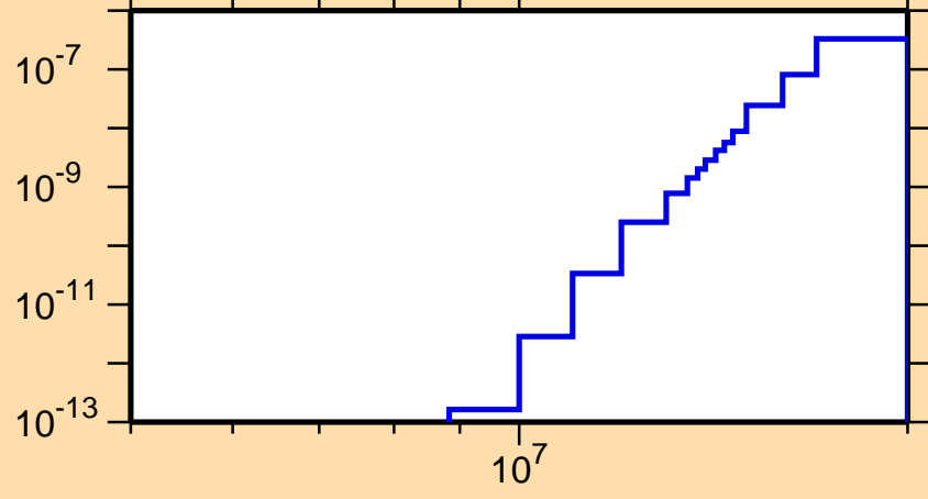
\sigma vs. E for ^{251}\text{No}(n,\text{He3})
