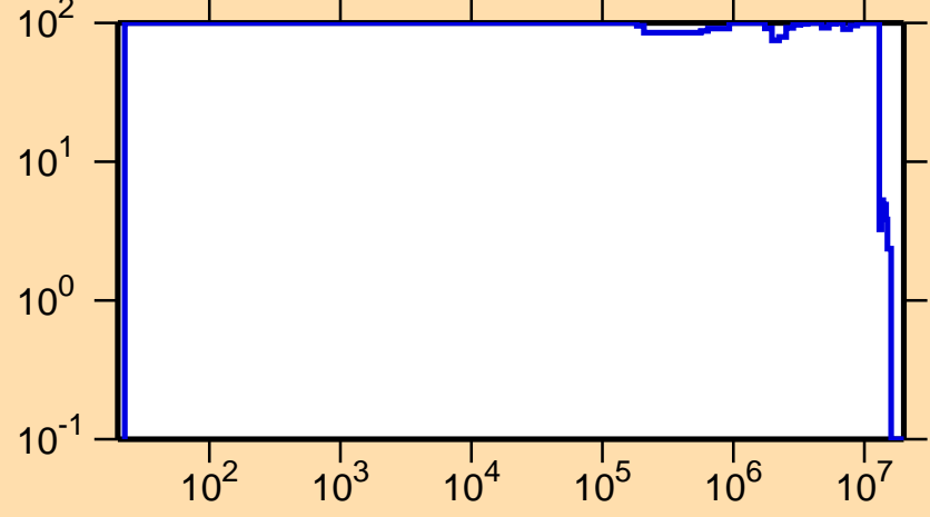
\Delta\sigma/\sigma vs. E for ^{251}\text{No}(n,n_1)
