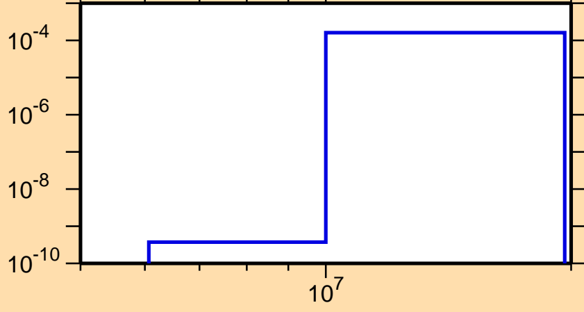
\sigma vs. E for ^{251}\text{No}(n,t)
