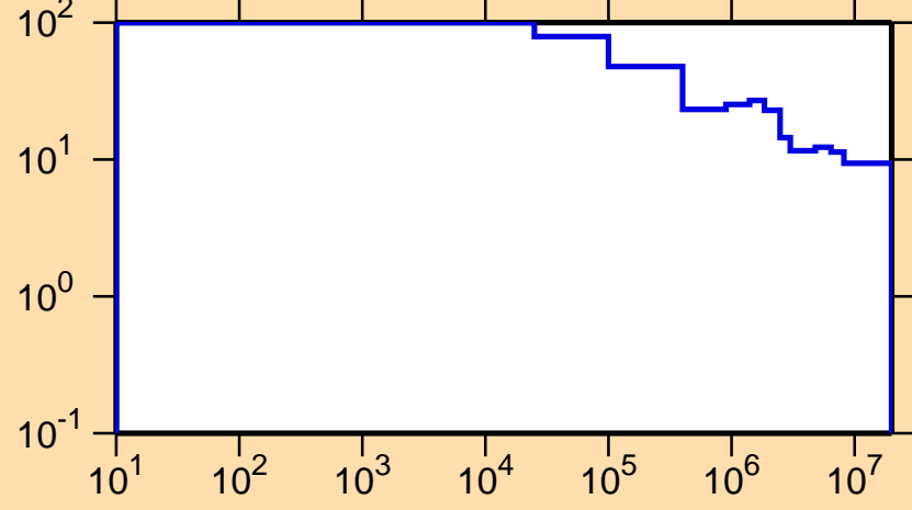
\Delta\sigma/\sigma vs. E for ^{251}\text{No}(n,\text{nonel.})
