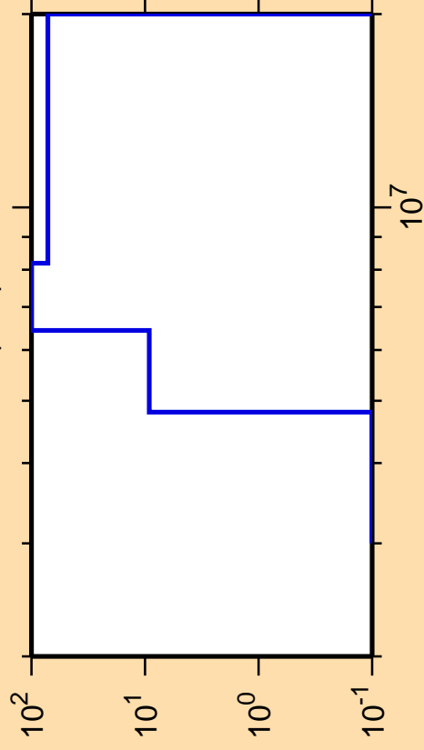
\Delta\sigma/\sigma vs. E for ^{251}\text{No}(n,d)
