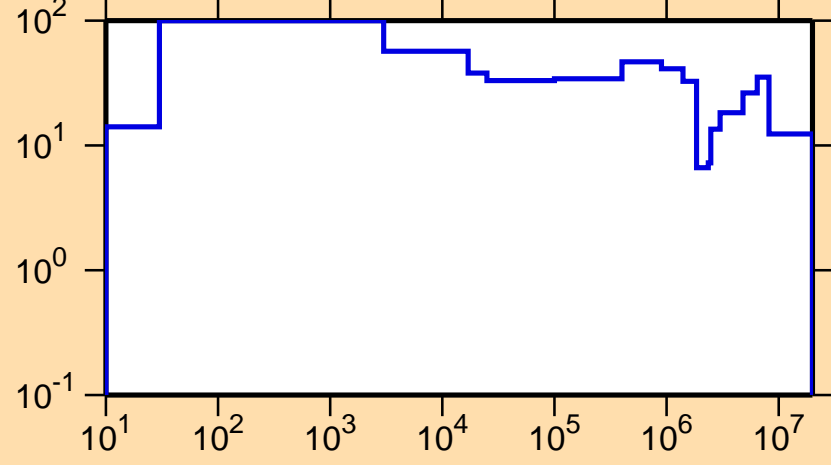
\Delta\sigma/\sigma vs. E for ^{251}\text{No}(n,\text{el.})
