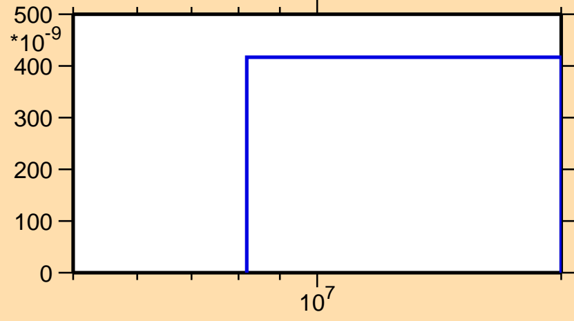
\sigma vs. E for ^{251}\text{No}(n,2np)
