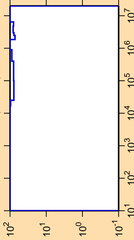
\Delta\sigma/\sigma vs. E for ^{251}\text{No}(n,\text{inel.})
