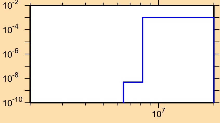
\sigma vs. E for ^{251}\text{No}(n,d)
