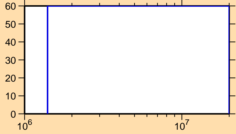
\Delta\sigma/\sigma vs. E for ^{251}\text{No}(n,ncont.)
