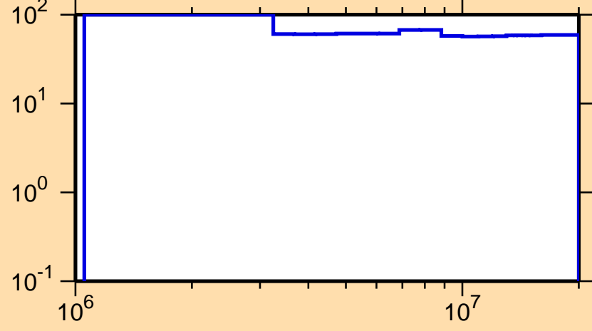
\Delta\sigma/\sigma vs. E for ^{253}\text{No}(n,n\text{cont.})
