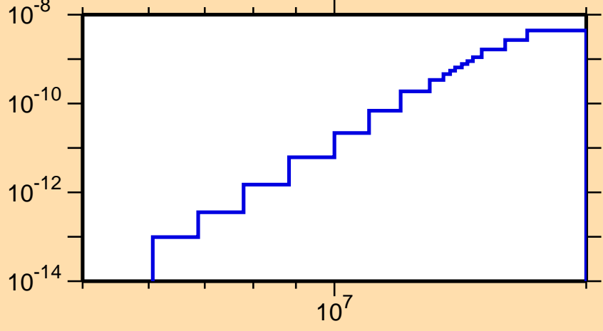
\sigma vs. E for ^{253}\text{No}(n,p\alpha)
