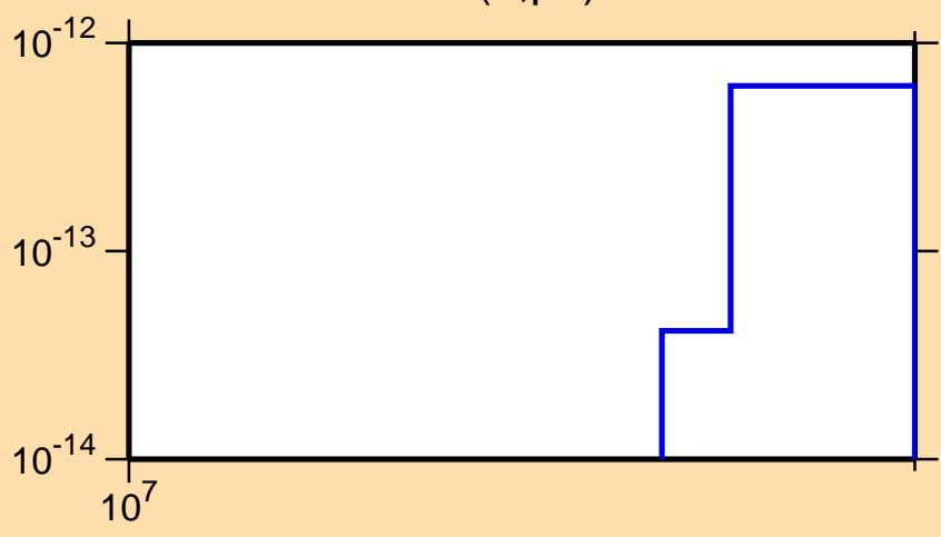
\sigma vs. E for ^{253}\text{No}(n,\text{pd})
