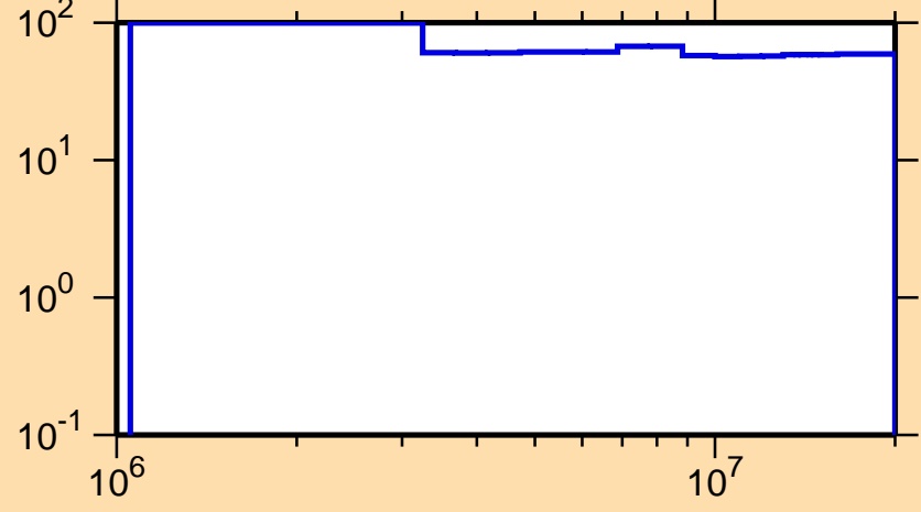
\Delta\sigma/\sigma vs. E for ^{253}\text{No}(n,ncont.)
