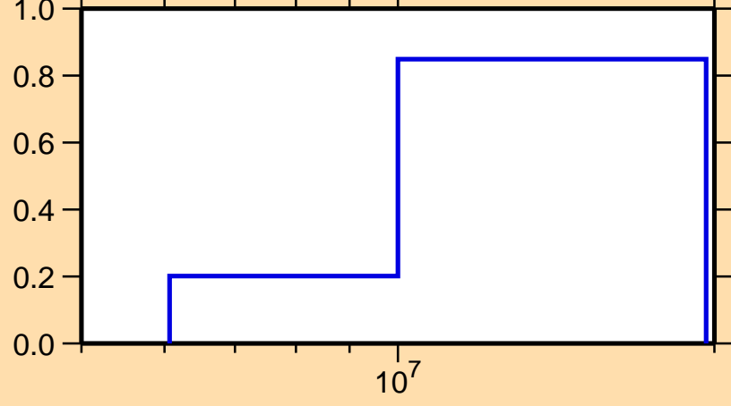
\sigma vs. E for ^{253}\text{No}(n,2n)
