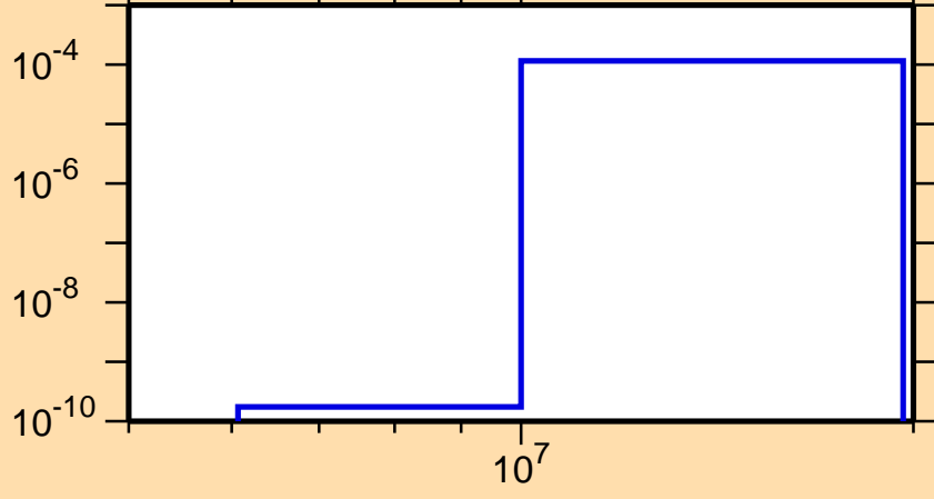
\sigma vs. E for ^{253}\text{No}(n,t)
