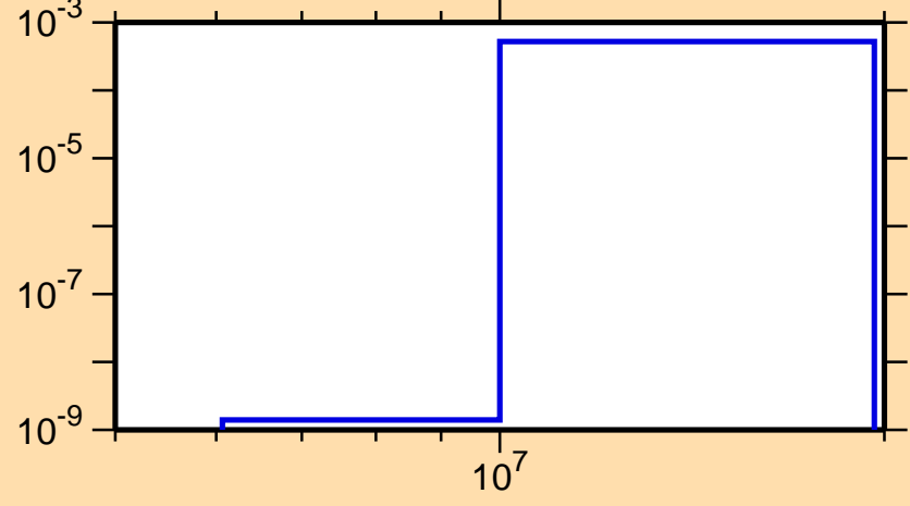
\sigma vs. E for ^{253}\text{No}(n,2n\alpha)
