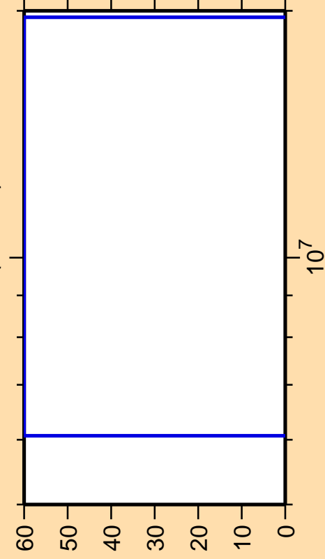
\Delta\sigma/\sigma vs. E for ^{253}\text{No}(n,2n\alpha)
