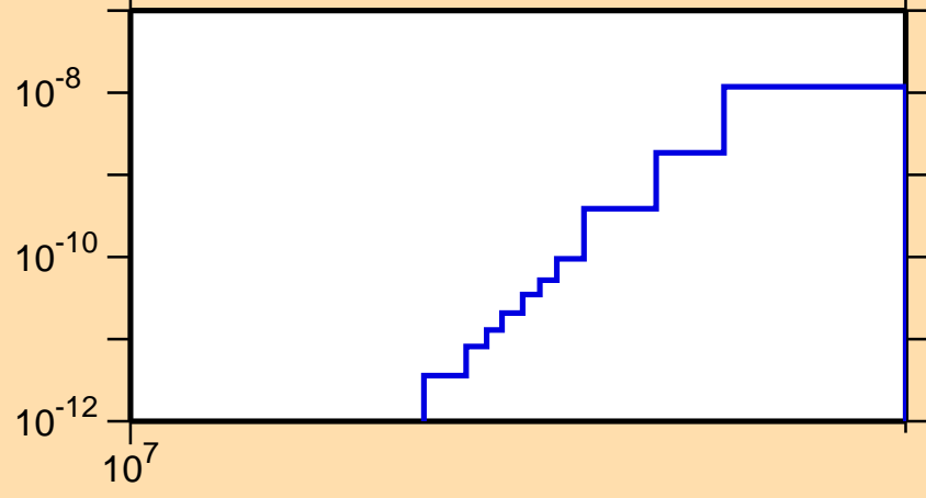
\sigma vs. E for ^{254}\text{No}(n,\text{He}3)
