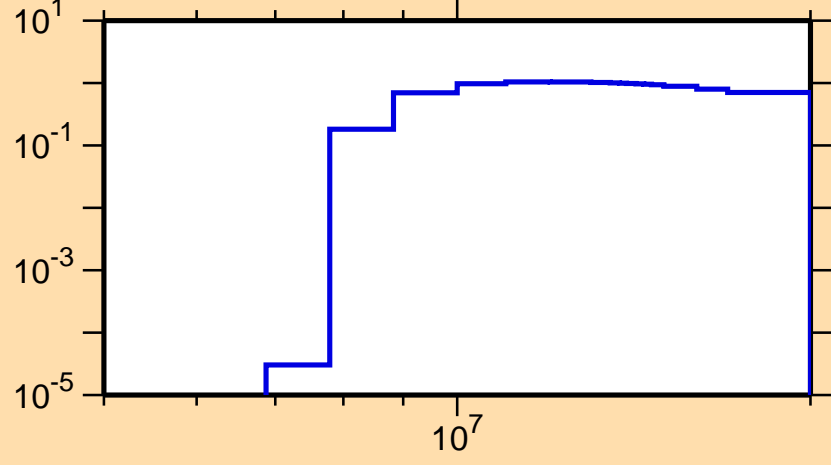
\sigma vs. E for ^{254}\text{No}(n,2n)
