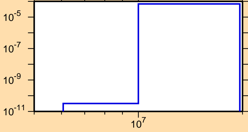
\sigma vs. E for ^{254}\text{No}(n,t)
