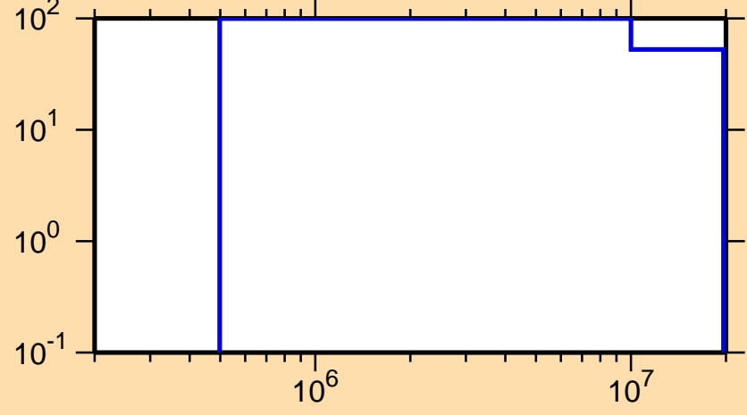
\Delta\sigma/\sigma vs. E for ^{254}\text{No}(n,f)
