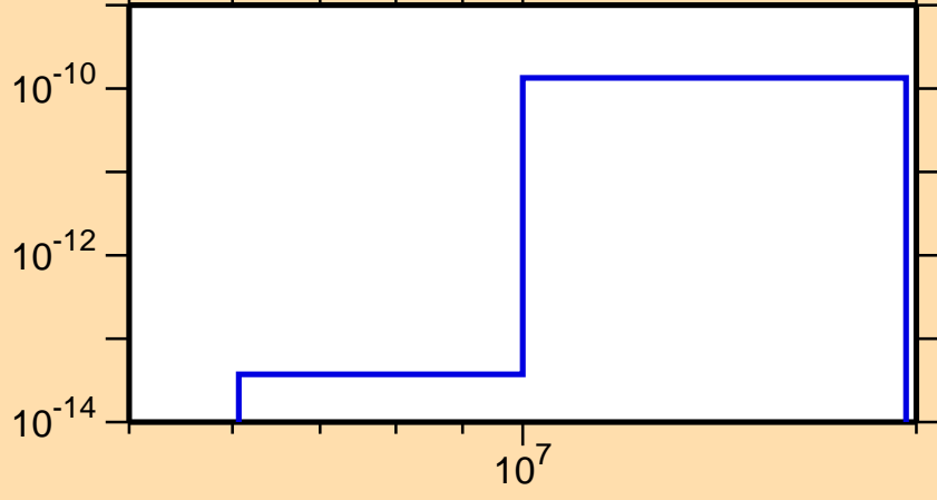
\sigma vs. E for ^{254}\text{No}(n,p\alpha)
