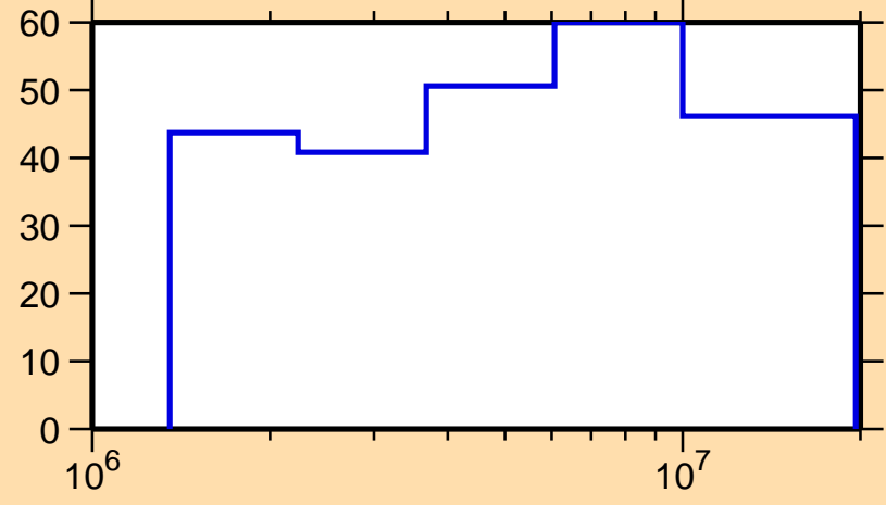
\Delta\sigma/\sigma vs. E for ^{256}\text{No}(n,ncont.)
