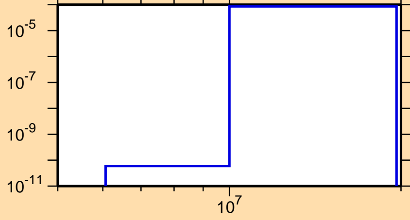
\sigma vs. E for ^{256}\text{No}(n,t)
