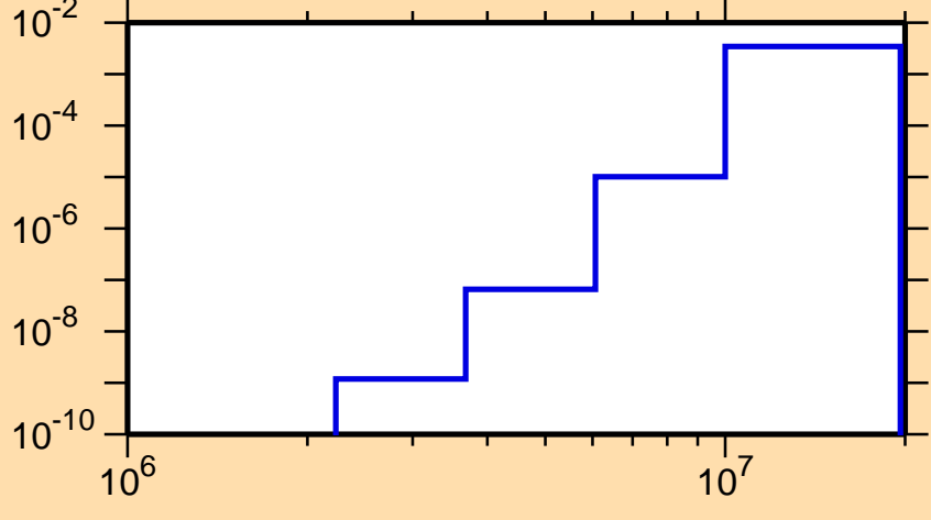
\sigma vs. E for ^{256}\text{No}(n,p)
