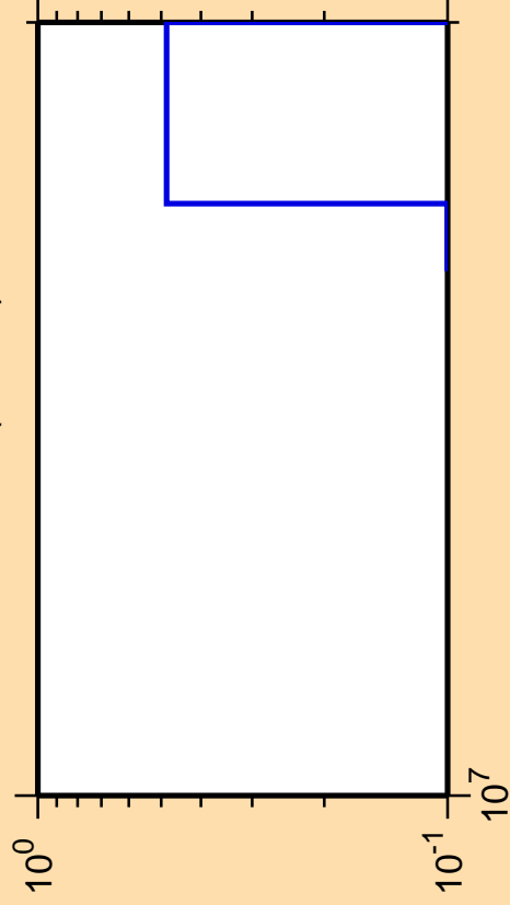
\Delta\sigma/\sigma vs. E for ^{257}\text{No}(\text{mt } 11)
