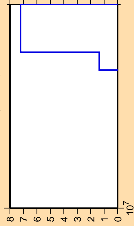
\Delta\sigma/\sigma vs. E for ^{257}\text{No}(\text{mt117})
