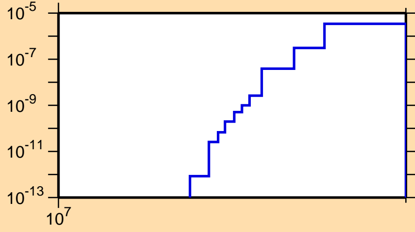
\sigma vs. E for ^{257}\text{No}(n,2np)
