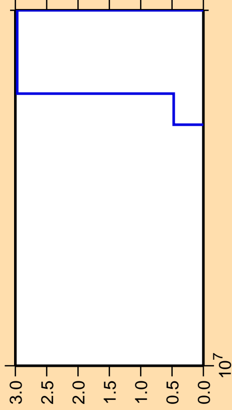
\Delta\sigma/\sigma vs. E for ^{257}\text{No}(\text{mt } 45)
