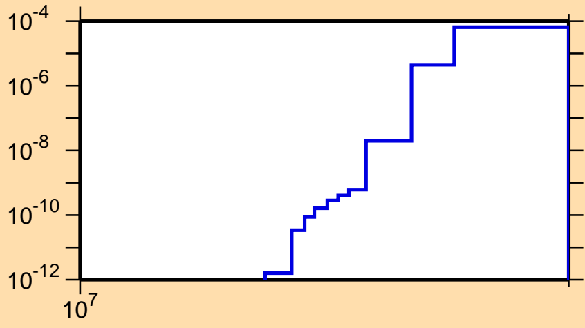
\sigma vs. E for ^{257}\text{No}(n,3n\alpha)
