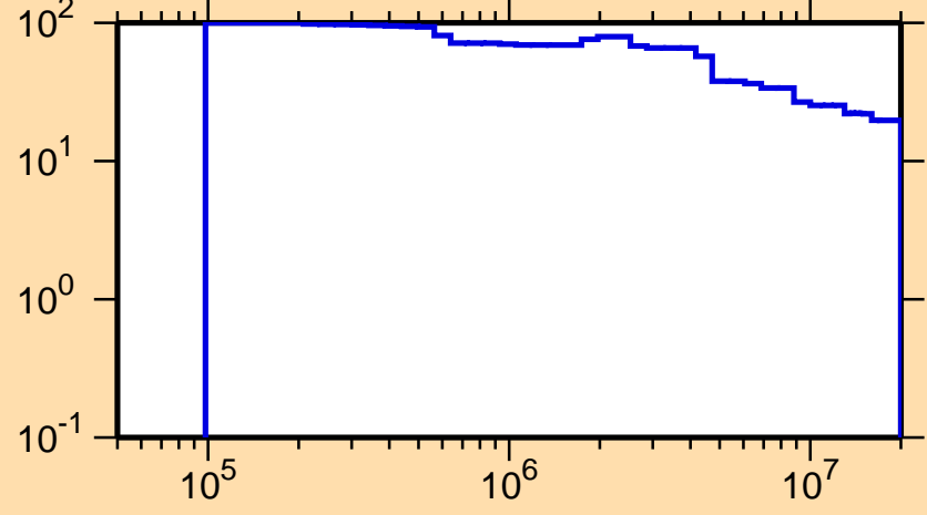
\Delta\sigma/\sigma vs. E for ^{257}\text{No}(n,f)
