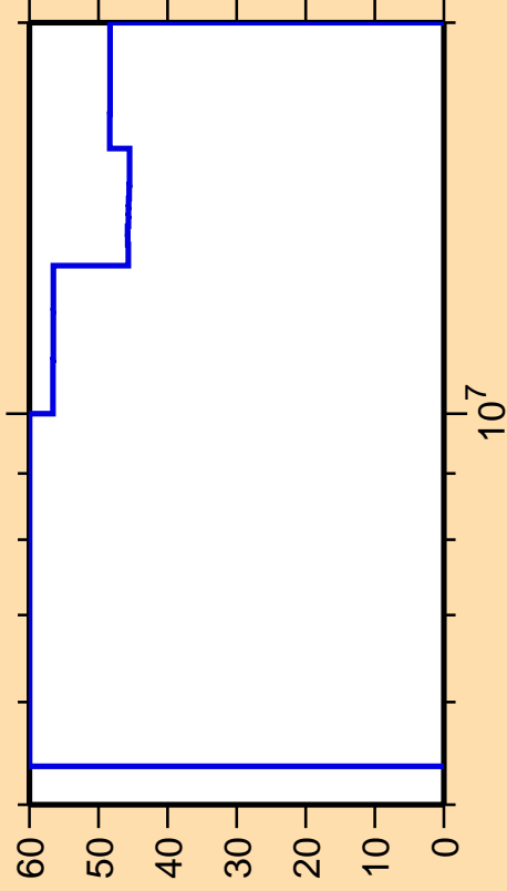
\Delta\sigma/\sigma vs. E for ^{257}\text{No}(n,p)
