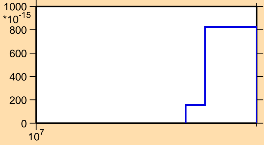
\sigma vs. E for ^{257}\text{No}(\text{mt117})
