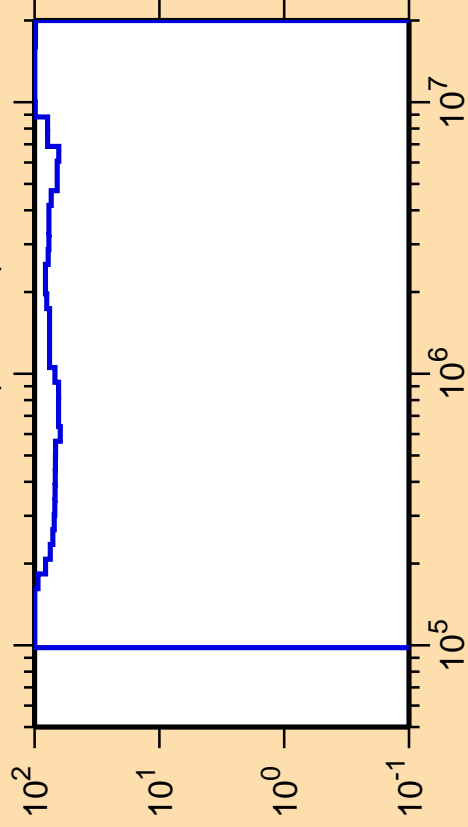
\Delta\sigma/\sigma vs. E for ^{257}\text{No}(n,\text{inel.})
