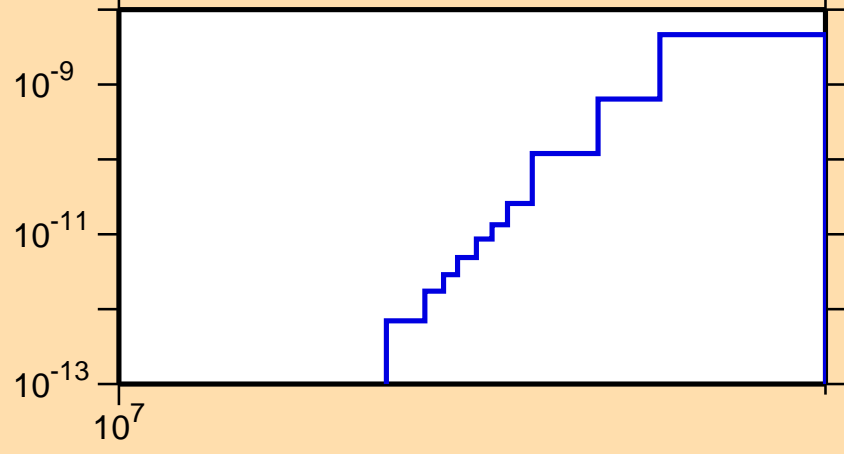
\sigma vs. E for ^{257}\text{No}(n,\text{He}3)
