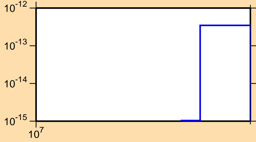
\sigma vs. E for ^{257}\text{No}(\text{mt } 11)
