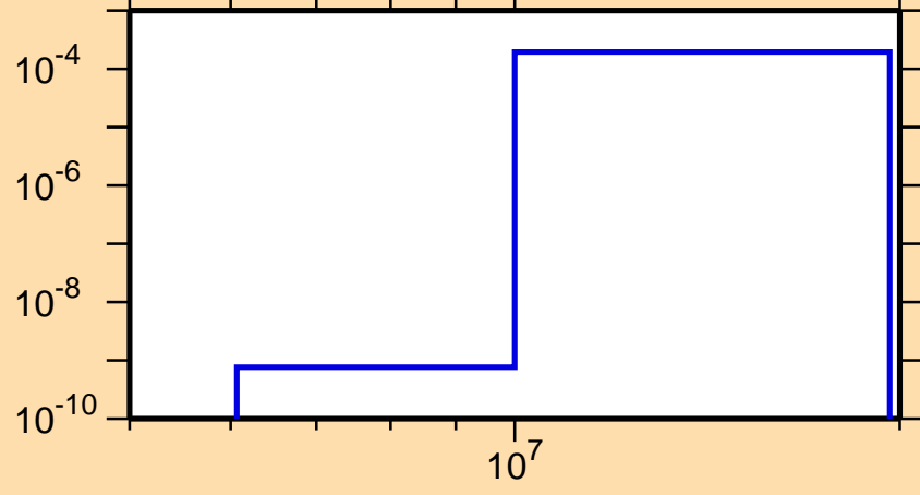
\sigma vs. E for ^{257}\text{No}(n,np)
