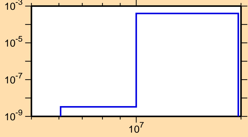
\sigma vs. E for ^{257}\text{No}(n,d)
