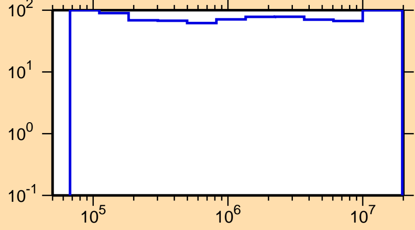
\Delta\sigma/\sigma vs. E for ^{257}\text{No}(n,\text{inel.})
