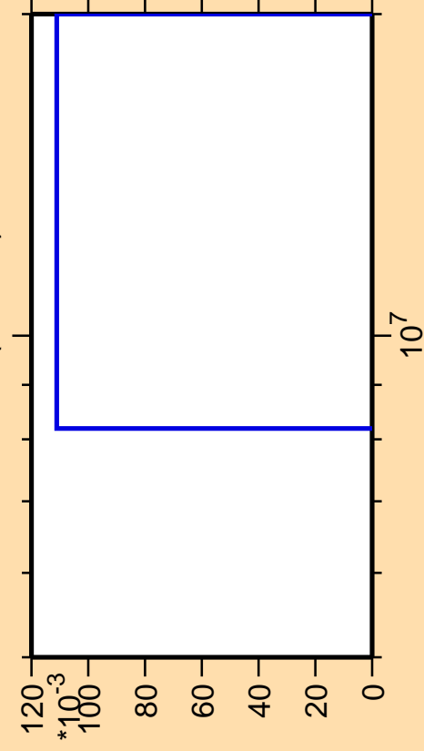
\Delta\sigma/\sigma vs. E for ^{257}\text{No}(\text{mt117})
