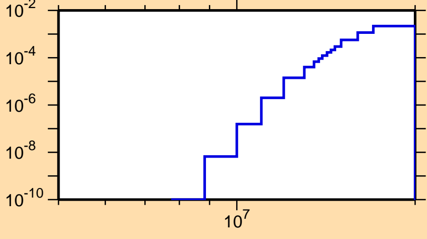
\sigma vs. E for ^{259}\text{No}(n,d)
