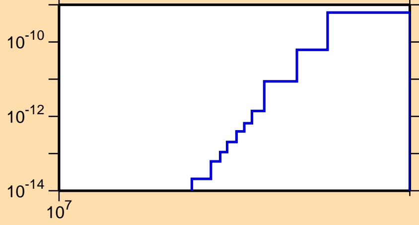
\sigma vs. E for ^{259}\text{No}(n,\text{He}3)
