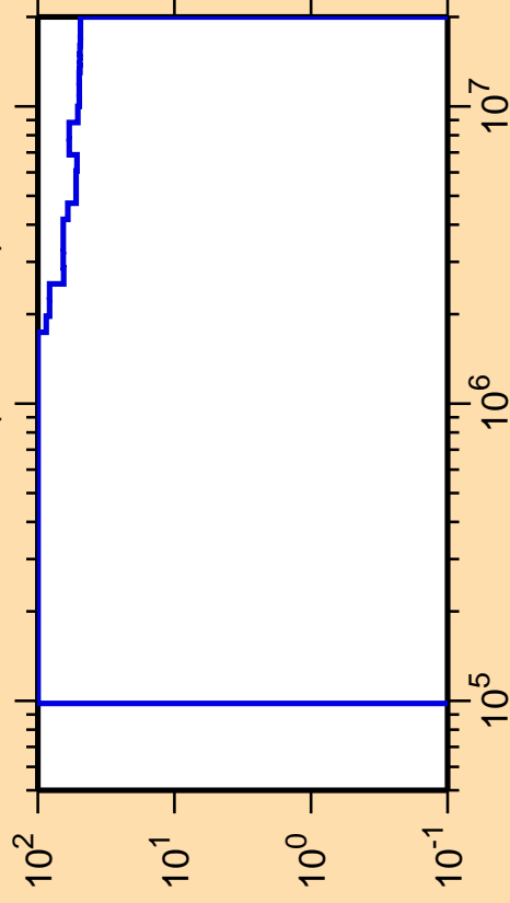
\Delta\sigma/\sigma vs. E for ^{259}\text{No}(n,\text{ncont.})
