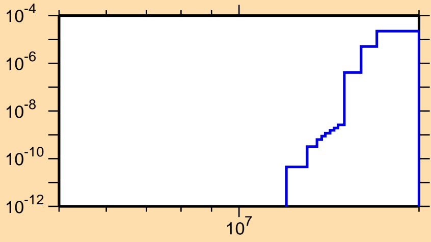
\sigma vs. E for ^{259}\text{No}(n,3n\alpha)
