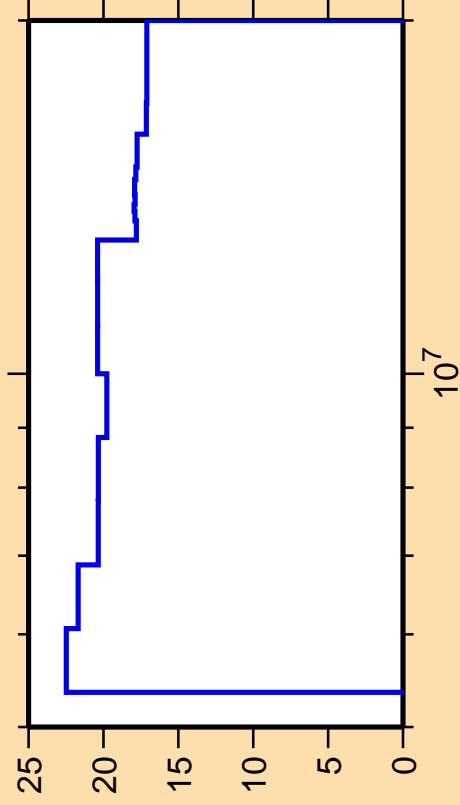
\Delta\sigma/\sigma vs. E for ^{259}\text{No}(n,f)
