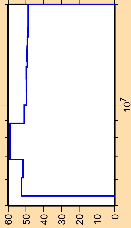
\Delta\sigma/\sigma vs. E for ^{259}\text{No}(n,n\text{cont.})
