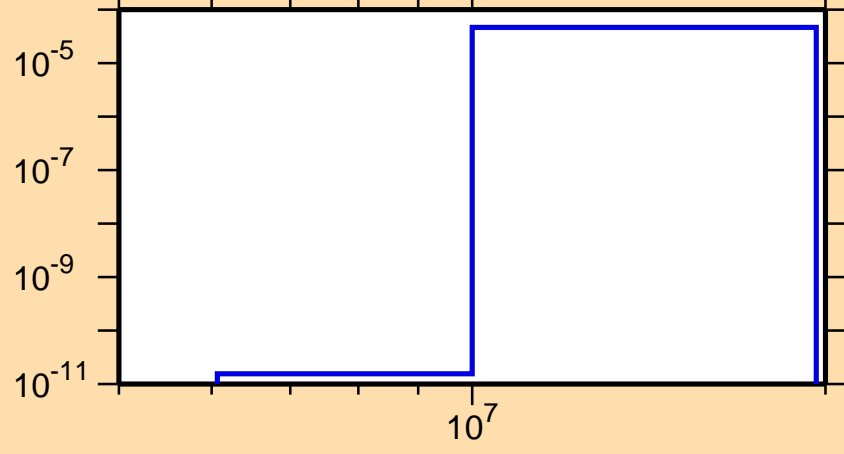
\sigma vs. E for ^{259}\text{No}(n,np)
