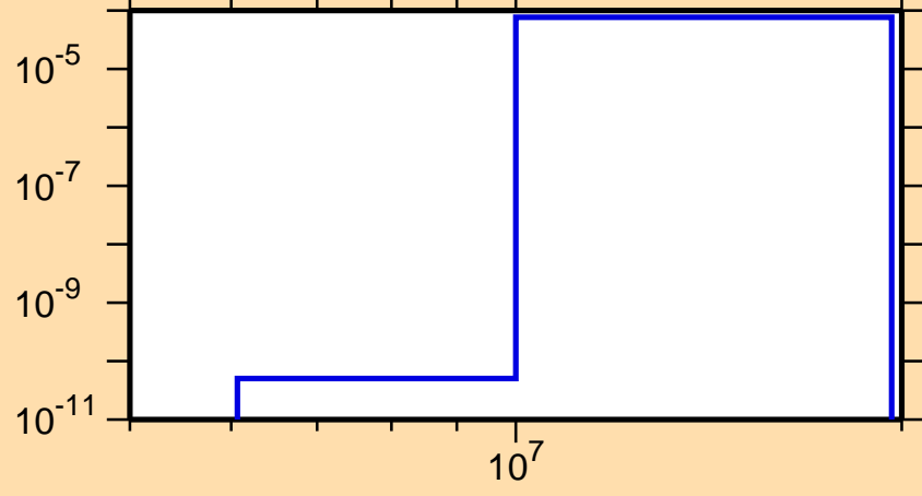
\sigma vs. E for ^{259}\text{No}(n,t)
