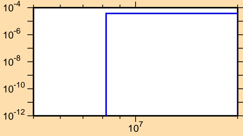
\sigma vs. E for ^{259}\text{No}(n,np)
