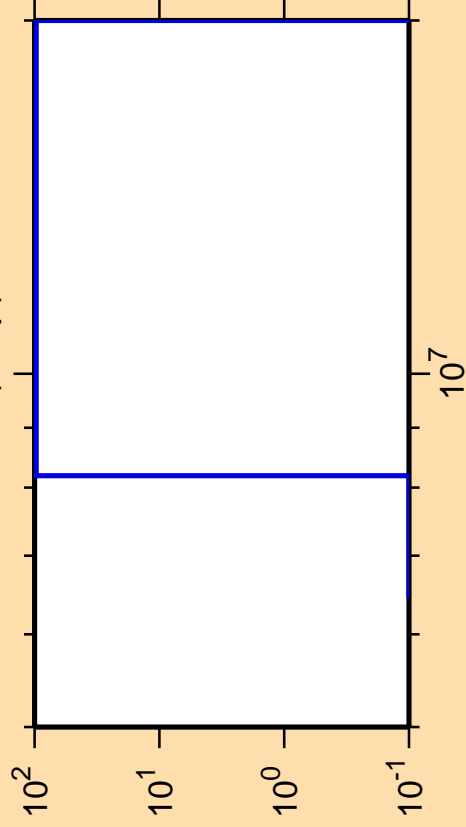
\Delta\sigma/\sigma vs. E for ^{259}\text{No}(n,np)
