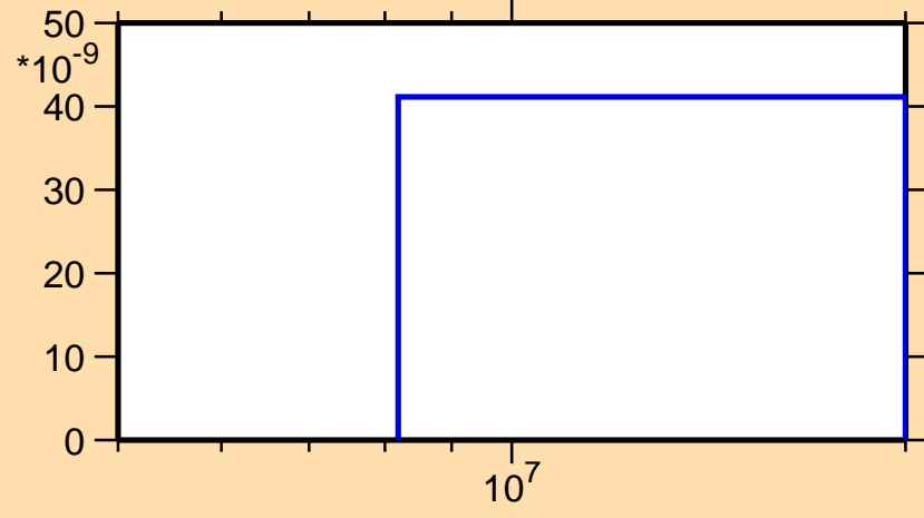
\sigma vs. E for ^{259}\text{No}(n,\text{nd})
