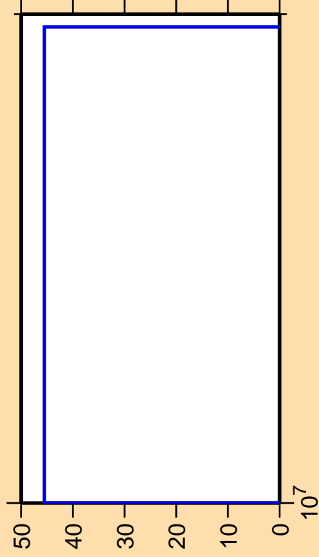
\Delta\sigma/\sigma vs. E for ^{261}\text{No}(n,\text{nt})
