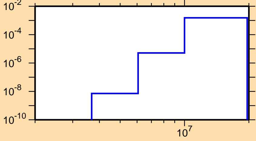
\sigma vs. E for ^{261}\text{No}(n,p)
