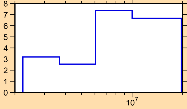
\Delta\sigma/\sigma vs. E for ^{261}\text{No}(n,\text{nonel.})
