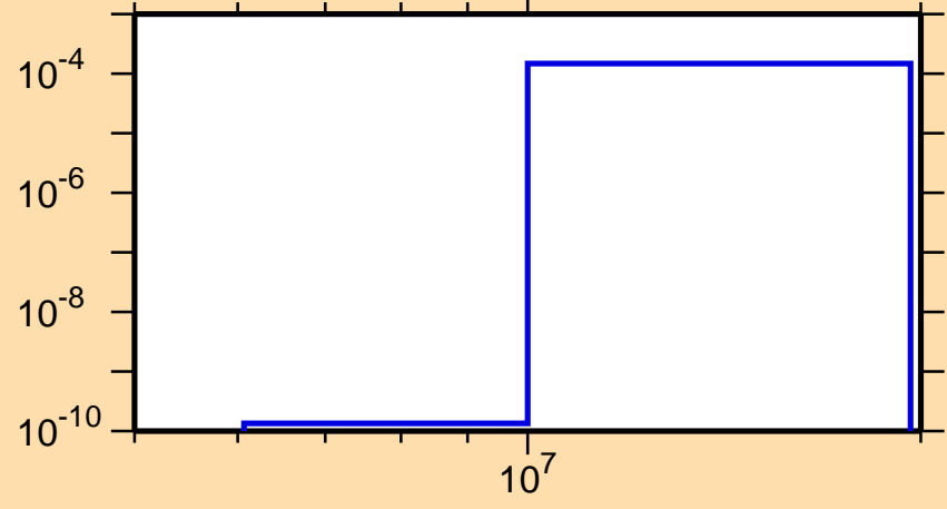
\sigma vs. E for ^{261}\text{No}(n,d)
