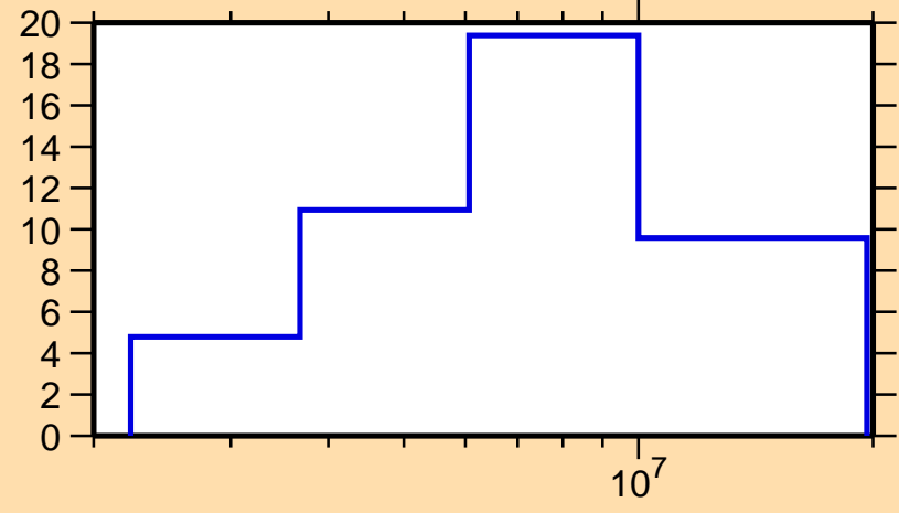
\Delta\sigma/\sigma vs. E for ^{261}\text{No}(n,el.)
