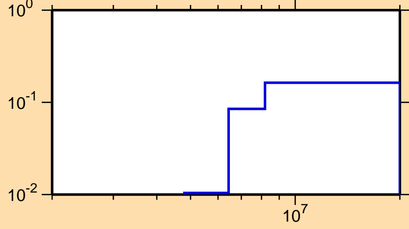
\sigma vs. E for ^{261}\text{No}(n,2n)
