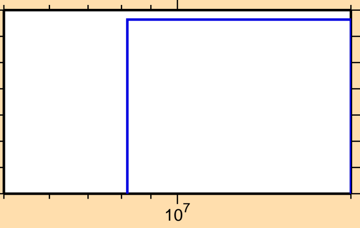
\sigma vs. E for ^{261}\text{No}(\text{mt } 11)
