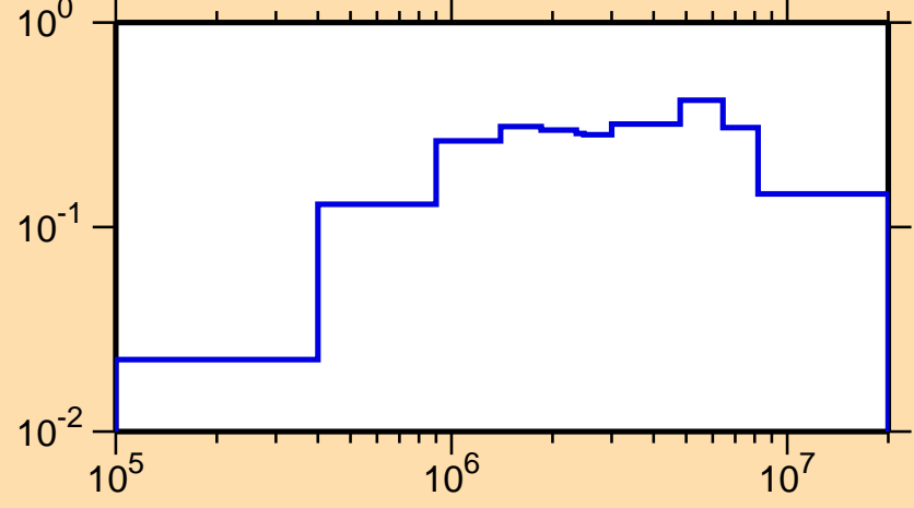
\sigma vs. E for ^{261}\text{No}(n,n\text{cont.})
