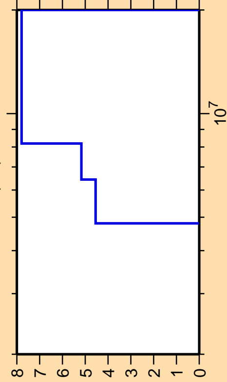
\Delta\sigma/\sigma vs. E for ^{261}\text{No}(n,f)
