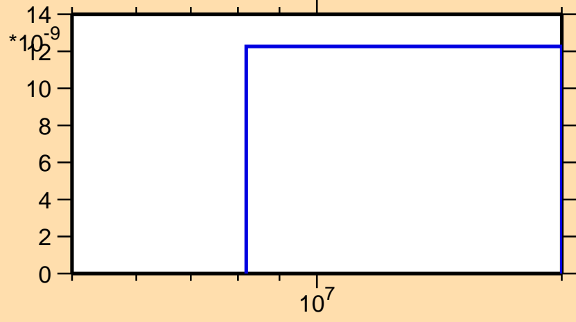
\sigma vs. E for ^{261}\text{No}(n,\text{nt})
