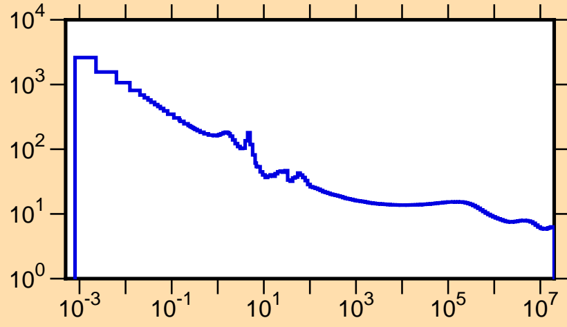
\sigma vs. E for ^{263}\text{No}(n,\text{tot.})
