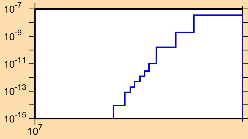
\sigma vs. E for ^{263}\text{No}(n,\text{nd})
