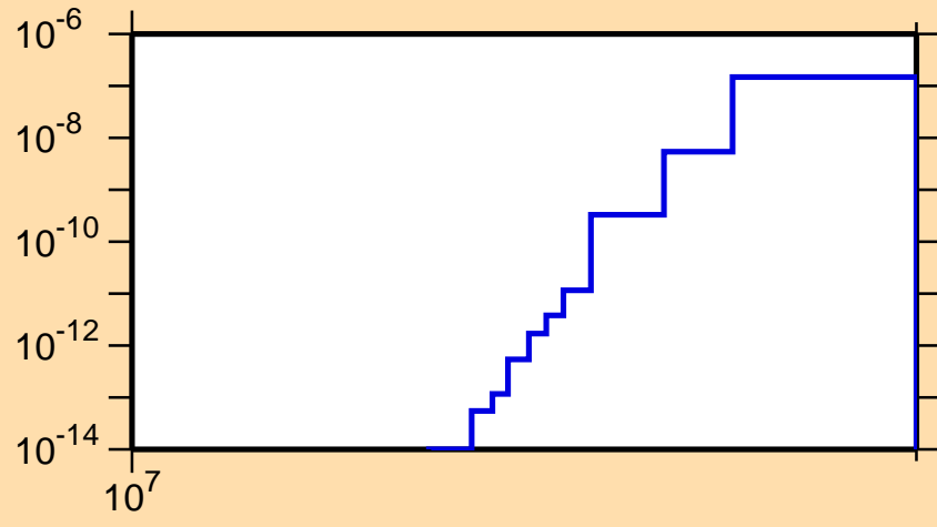
\sigma vs. E for ^{263}\text{No}(n,nt)
