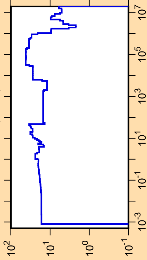
\Delta\sigma/\sigma vs. E for ^{263}\text{No}(n,\text{tot.})
