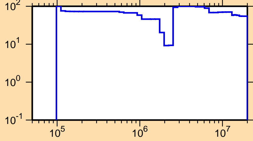
\Delta\sigma/\sigma vs. E for ^{264}\text{No}(n,n_1)
