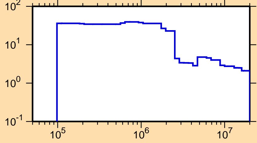
\Delta\sigma/\sigma vs. E for ^{264}\text{No}(n,\text{nonel.})
