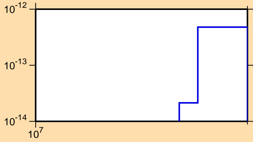
\sigma vs. E for ^{264}\text{No}(n,\text{He}3)
