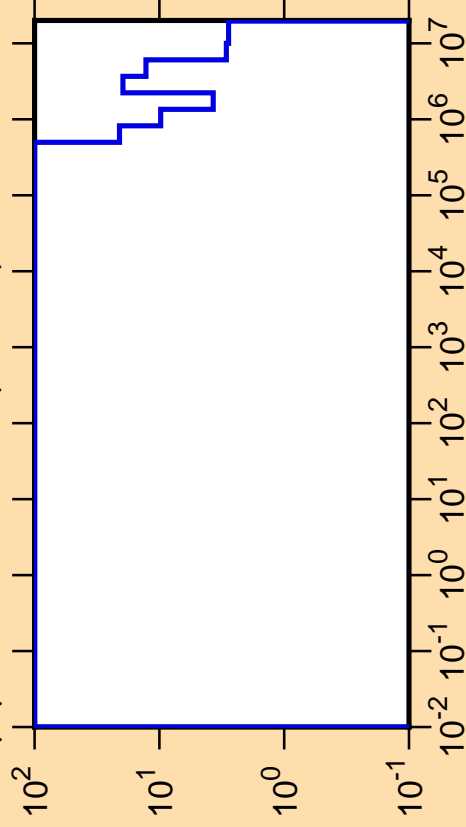
\Delta\mu/\mu vs. E for ^{264}\text{No}(\text{mt251})
