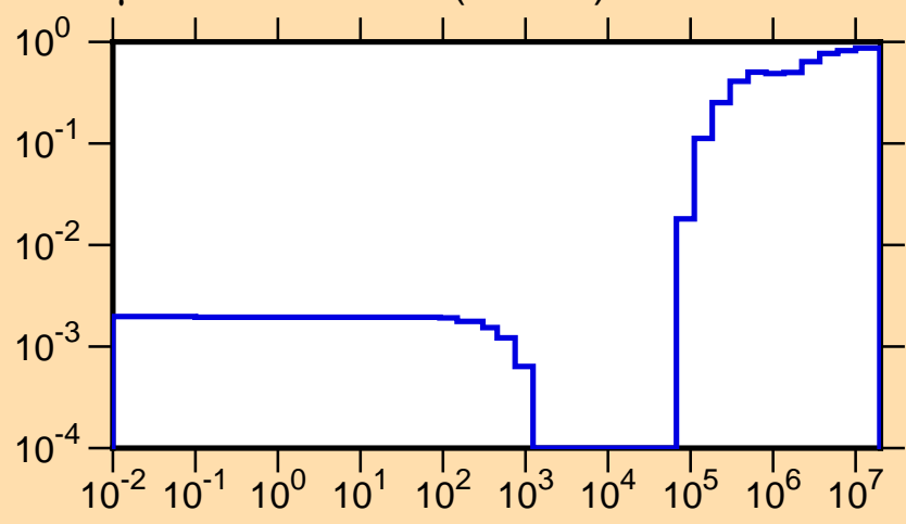
\mu vs. E for ^{264}\text{No}(\text{mt251})
