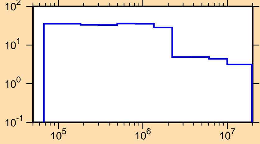
\Delta\sigma/\sigma vs. E for ^{264}\text{No}(n,f)
