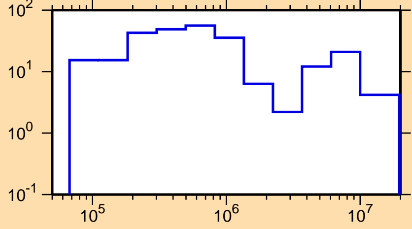
\Delta\sigma/\sigma vs. E for ^{264}\text{No}(n,\text{el.})
