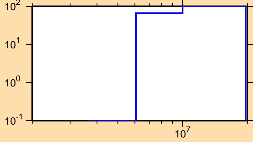
\Delta\sigma/\sigma vs. E for ^{264}\text{No}(n,p)
