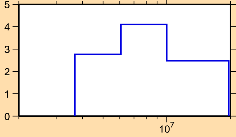
\Delta\sigma/\sigma vs. E for ^{264}\text{No}(n,\text{nonel.})
