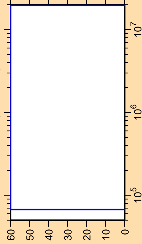
\Delta\sigma/\sigma vs. E for ^{264}\text{No}(n,\text{ncont.})
