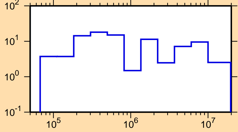
\Delta\sigma/\sigma vs. E for ^{264}\text{No}(n,\text{tot.})
