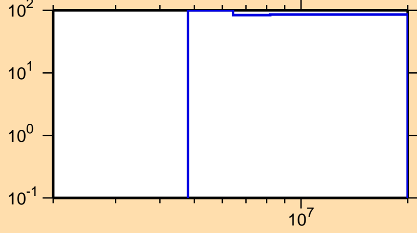
\Delta\sigma/\sigma vs. E for ^{264}\text{No}(n,2n)
