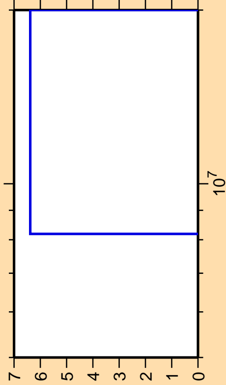
\Delta\sigma/\sigma vs. E for ^{264}\text{No}(n,2np)
