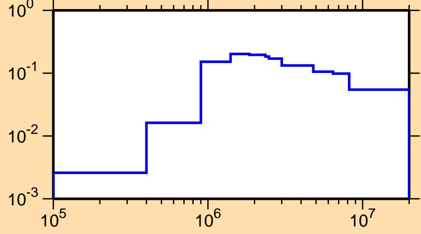
\sigma vs. E for ^{264}\text{No}(n,n\text{cont.})
