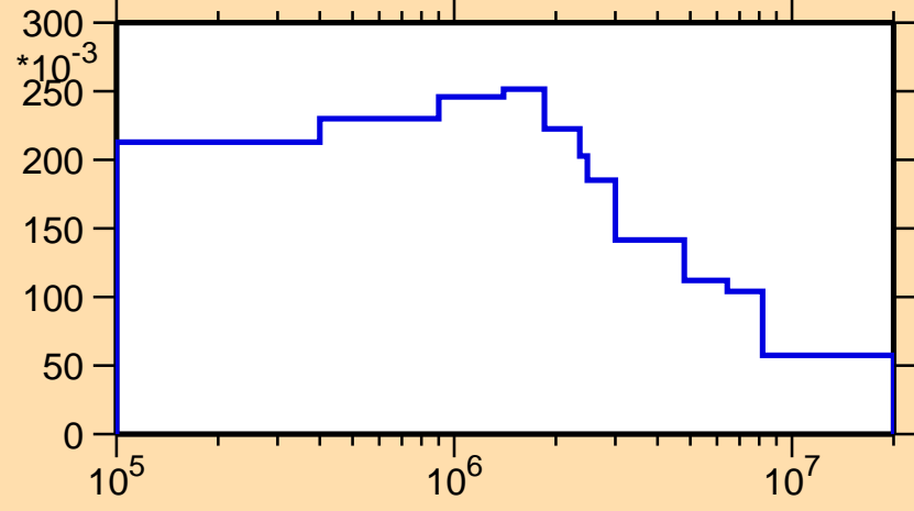
\sigma vs. E for ^{264}\text{No}(n,\text{inel.})
