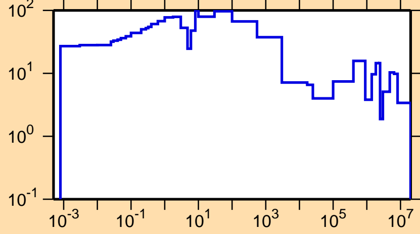
\Delta\sigma/\sigma vs. E for ^{264}\text{No}(n,tot.)
