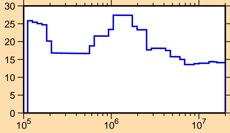
\Delta\sigma/\sigma vs. E for ^{228}\text{Np}(n,n\text{nonel.})
