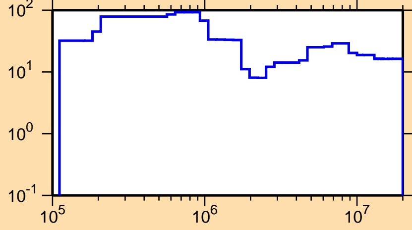
\Delta\sigma/\sigma vs. E for ^{228}\text{Np}(n,\text{el.})
