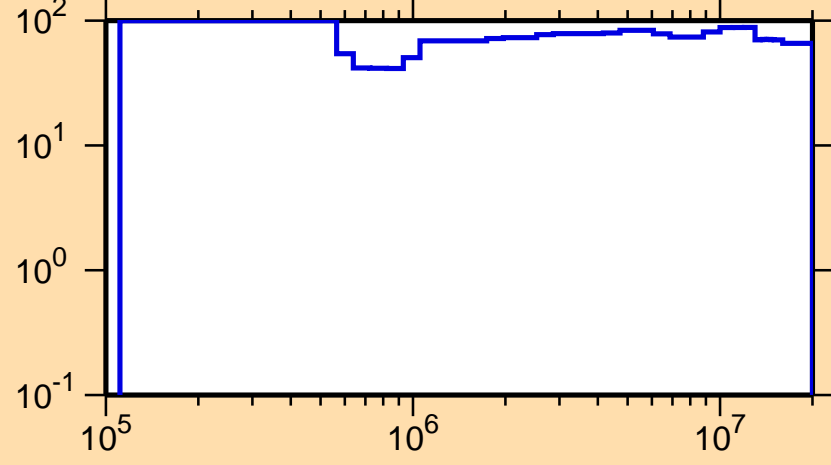
\Delta\sigma/\sigma vs. E for ^{228}\text{Np}(n,\text{inel.})
