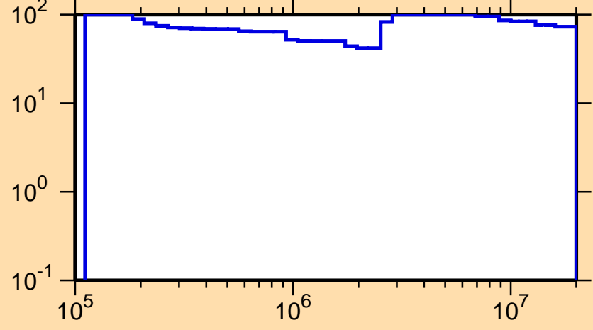
\Delta\sigma/\sigma vs. E for ^{228}\text{Np}(n,n_1)
