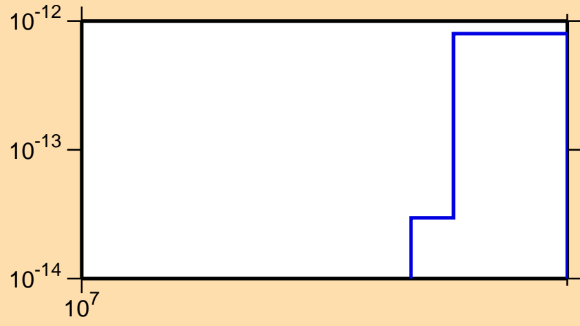
\sigma vs. E for ^{228}\text{Np}(n,\text{pt})
