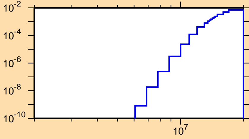
\sigma vs. E for ^{228}\text{Np}(n,d)
