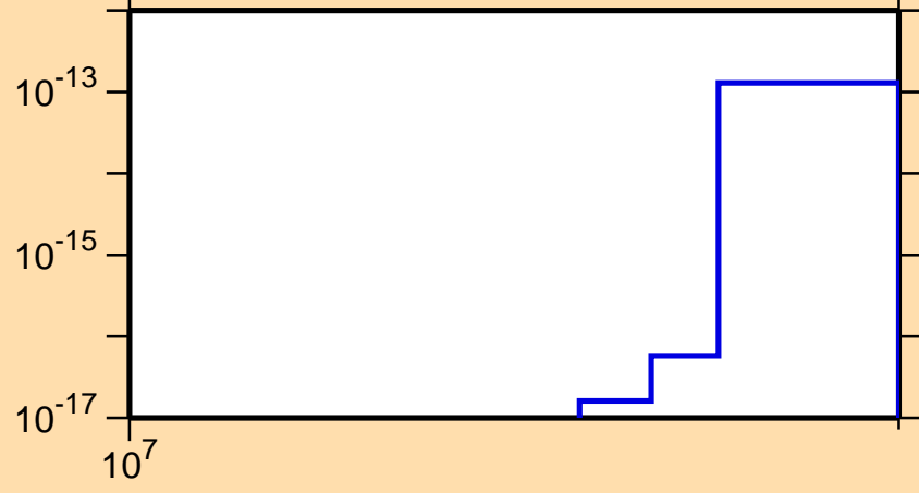
\sigma vs. E for ^{228}\text{Np}(\text{mt } 11)
