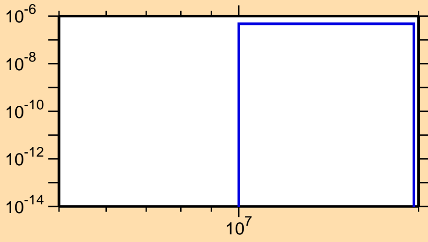
\sigma vs. E for ^{228}\text{Np}(n,\text{nd})
