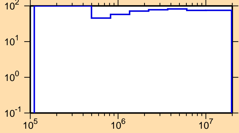
\Delta\sigma/\sigma vs. E for ^{228}\text{Np}(n,ncont.)
