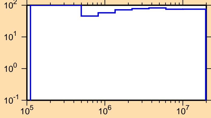
\Delta\sigma/\sigma vs. E for ^{228}\text{Np}(n,n\text{cont.})
