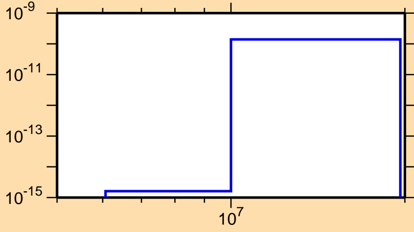
\sigma vs. E for ^{228}\text{Np}(\text{mt } 45)
