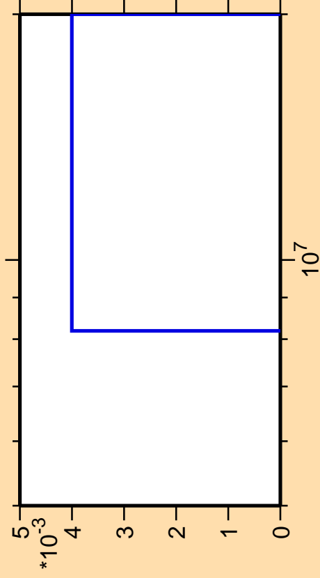
\Delta\sigma/\sigma vs. E for ^{228}\text{Np}(\text{mt } 11)
