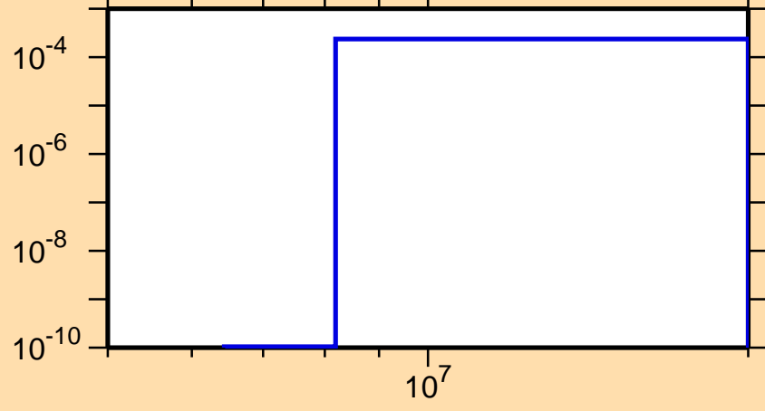
\sigma vs. E for ^{228}\text{Np}(n,t)
