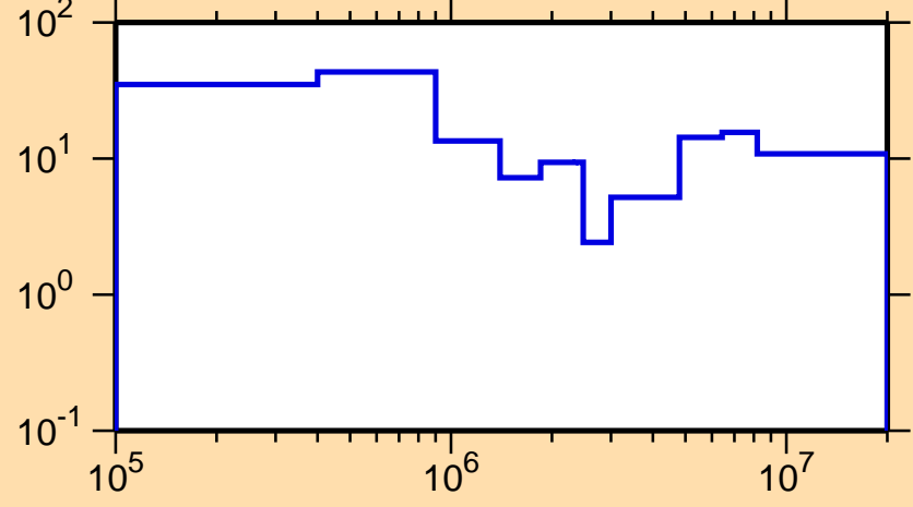
\Delta\sigma/\sigma vs. E for ^{228}\text{Np}(n,\text{tot.})
