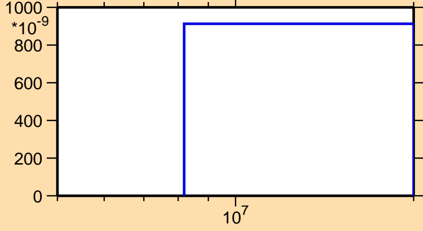
\sigma vs. E for ^{228}\text{Np}(n,2np)
