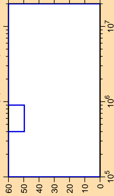
\Delta\sigma/\sigma vs. E for ^{228}\text{Np}(n,\text{ncont.})
