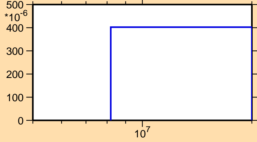
\sigma vs. E for ^{228}\text{Np}(n,3n)
