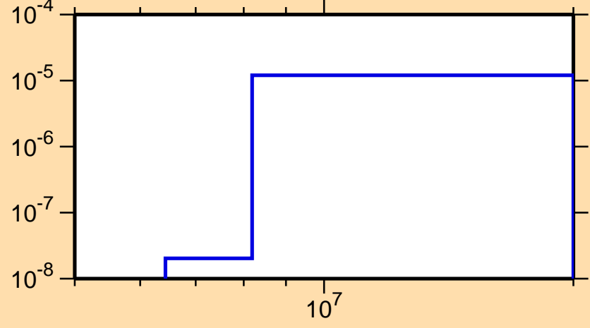
\sigma vs. E for ^{228}\text{Np}(n,2n\alpha)
