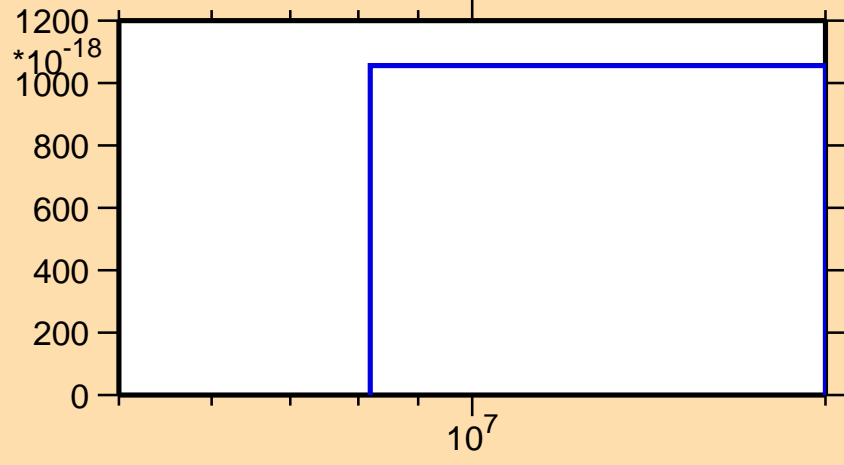
\sigma vs. E for ^{228}\text{Np}(\text{mt } 11)
