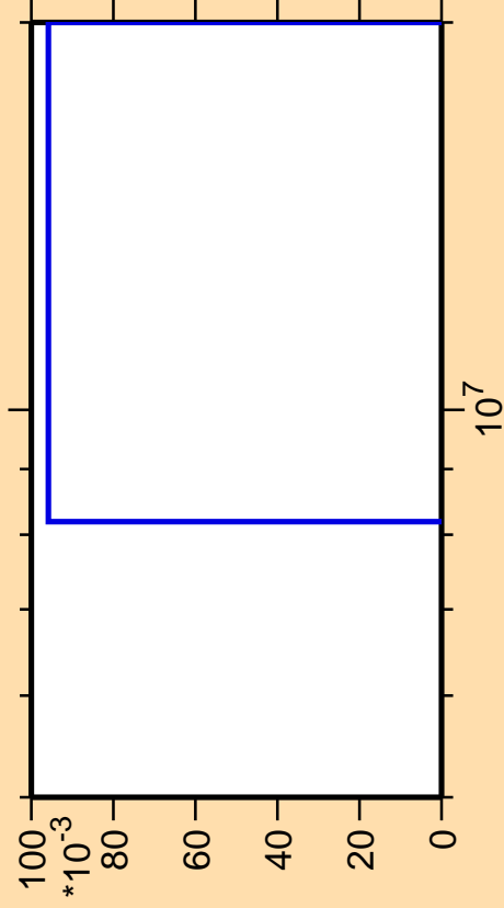
\Delta\sigma/\sigma vs. E for ^{228}\text{Np}(n,\text{pd})
