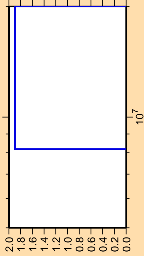
\Delta\sigma/\sigma vs. E for ^{228}\text{Np}(\text{mt } 34)
