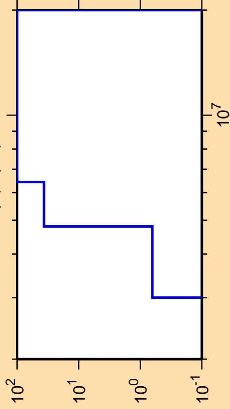
\Delta\sigma/\sigma vs. E for ^{228}\text{Np}(n,p\alpha)
