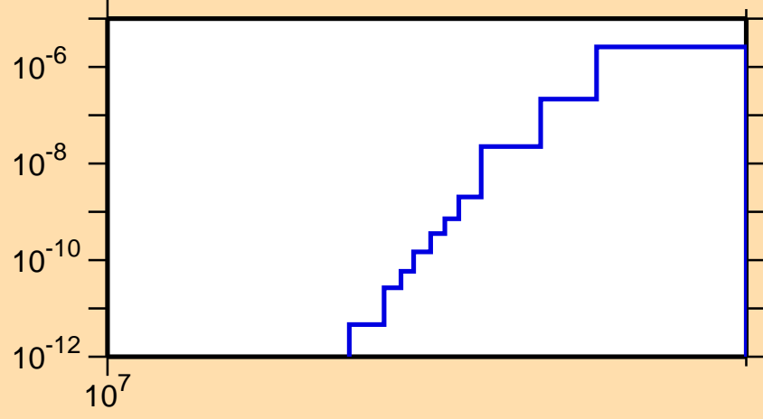
\sigma vs. E for ^{229}\text{Np}(n,\text{nd})
