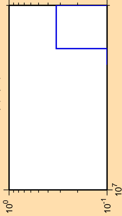
\Delta\sigma/\sigma vs. E for ^{229}\text{Np}(n,pd)
