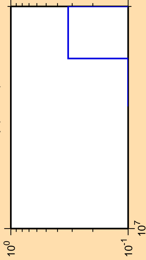
\Delta\sigma/\sigma vs. E for ^{229}\text{Np}(\text{mt } 11)
