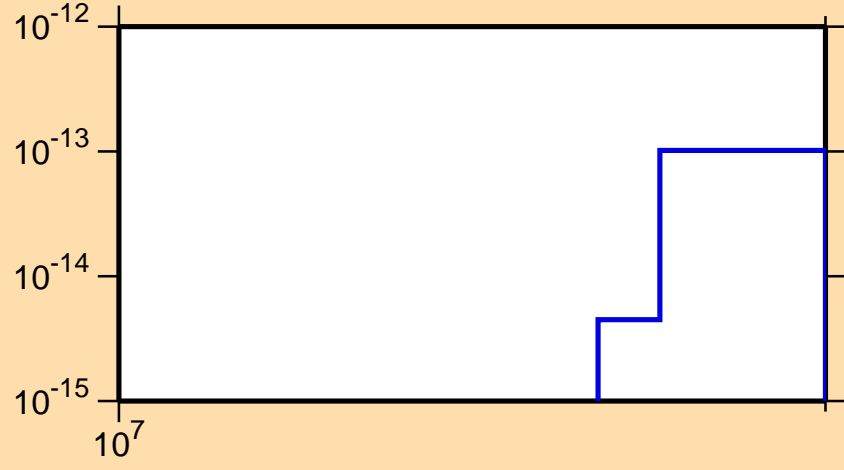
\sigma vs. E for ^{229}\text{Np}(n,pd)
