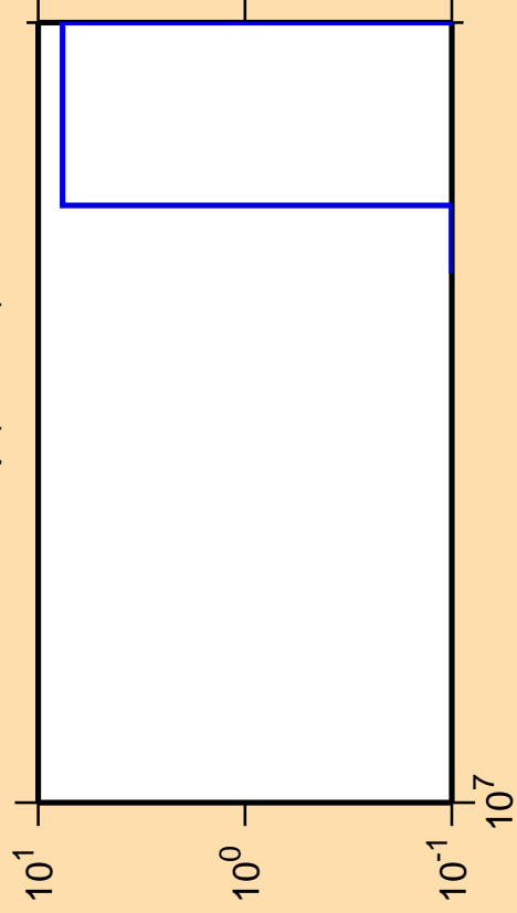
\Delta\sigma/\sigma vs. E for ^{229}\text{Np} (mt 34)
