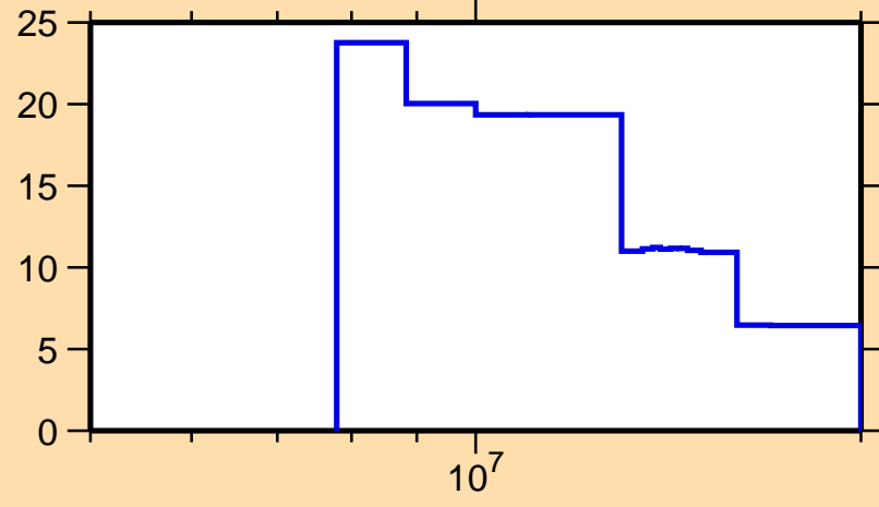
\Delta\sigma/\sigma vs. E for ^{229}\text{Np}(n,\text{tot.})
