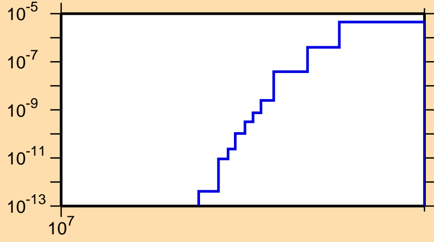
\sigma vs. E for ^{229}\text{Np}(n,2np)
