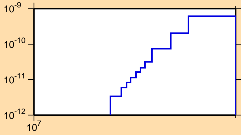
\sigma vs. E for ^{229}\text{Np}(\text{mt } 45)
