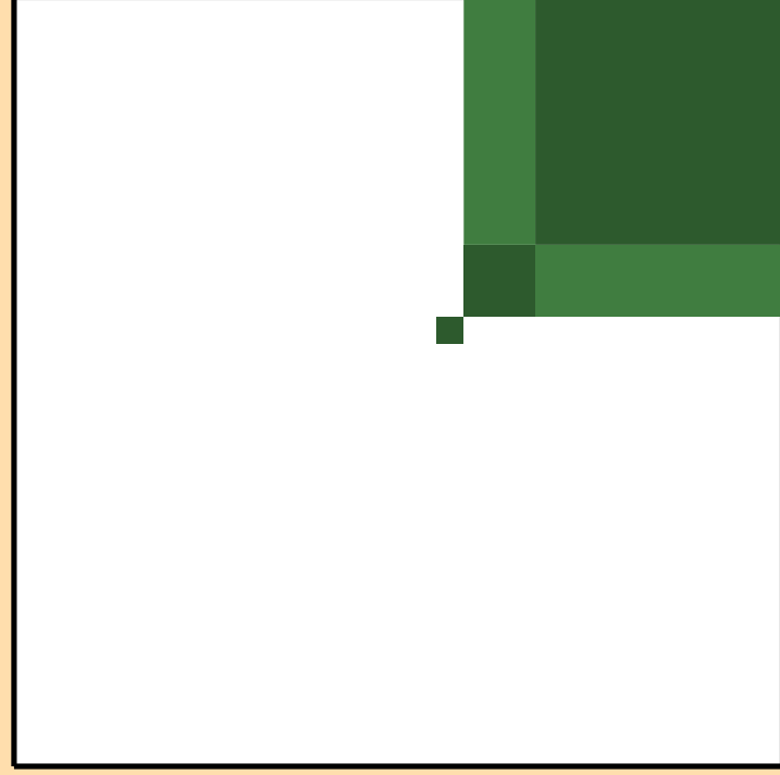
\sigma vs. E for ^{229}\text{Np}(n,3n)
