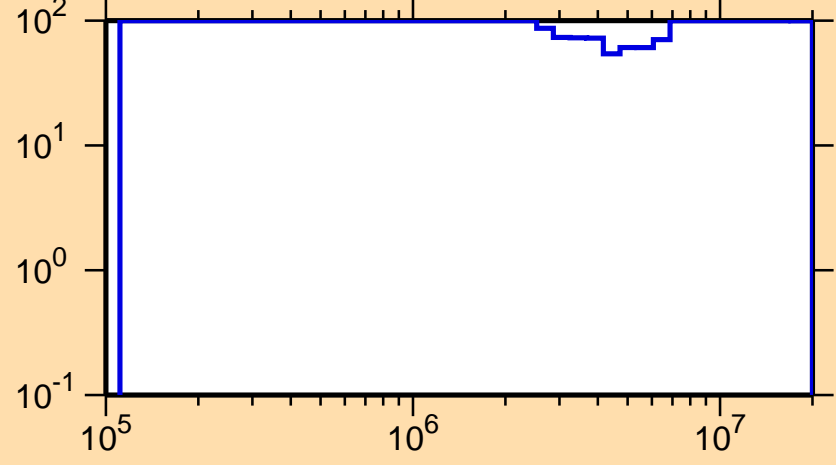
\Delta\sigma/\sigma vs. E for ^{229}\text{Np}(n,ncont.)
