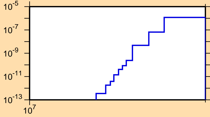
\sigma vs. E for ^{229}\text{Np}(n,nt)
