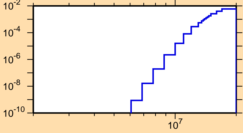
\sigma vs. E for ^{229}\text{Np}(n,d)
