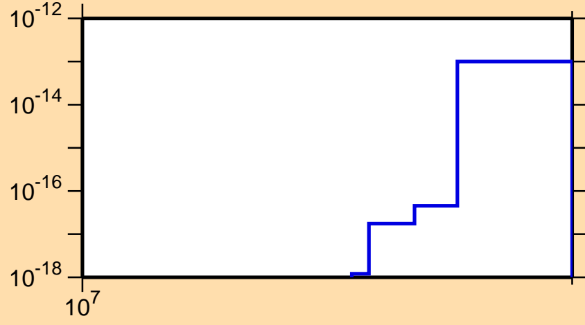
\sigma vs. E for ^{229}\text{Np}(\text{mt } 11)
