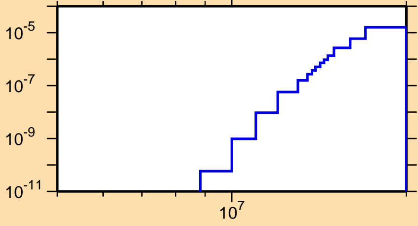
\sigma vs. E for ^{229}\text{Np}(n,2n\alpha)
