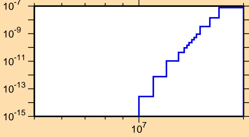
\sigma vs. E for ^{229}\text{Np}(n,\text{He}3)
