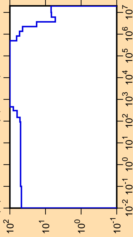
\Delta\mu/\mu vs. E for ^{229}\text{Np}(\text{mt251})
