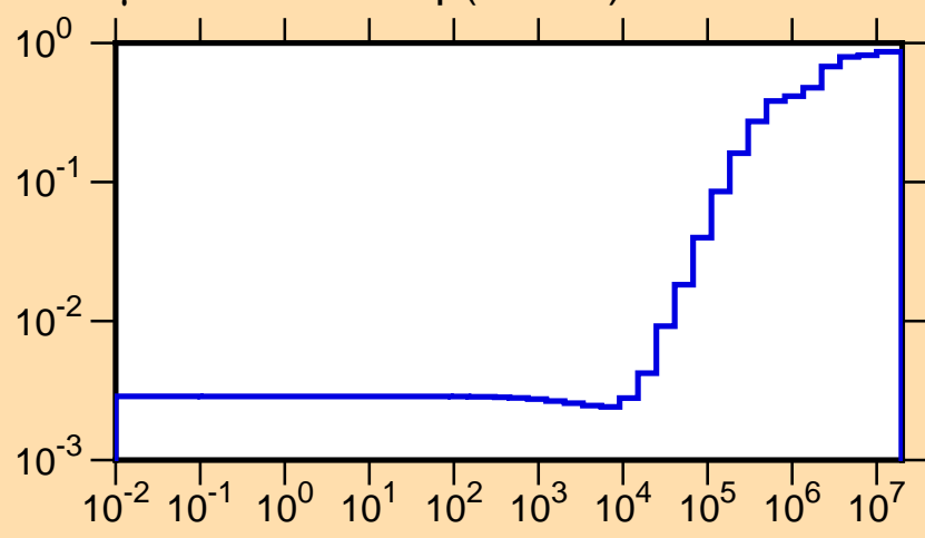
\mu vs. E for ^{229}\text{Np}(\text{mt251})
