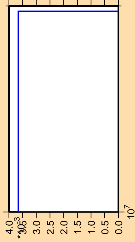
\Delta\sigma/\sigma vs. E for ^{229}\text{Np}(n,\text{pd})
