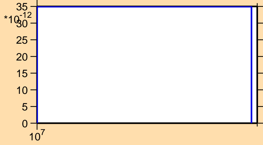
\sigma vs. E for ^{229}\text{Np} (mt 45)
