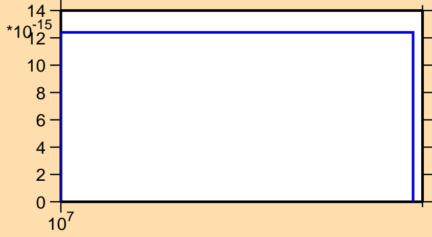
\sigma vs. E for ^{229}\text{Np} (mt 34)
