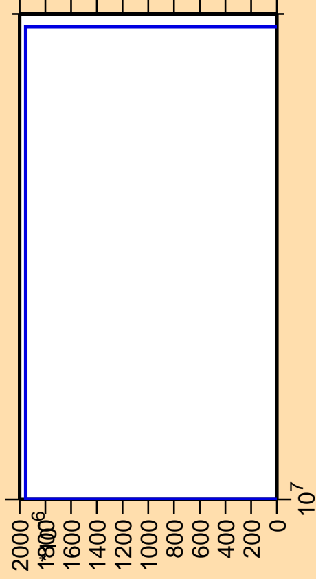
\Delta\sigma/\sigma vs. E for ^{229}\text{Np} (mt 11)
