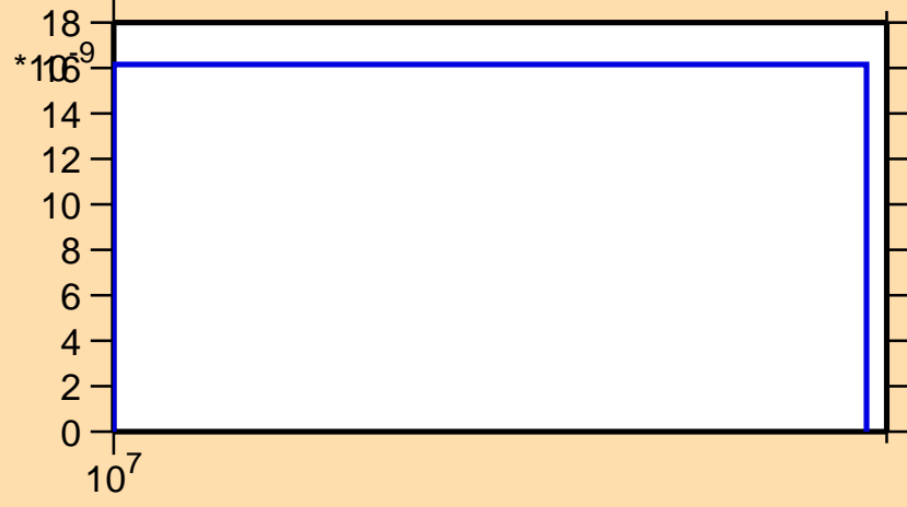
\sigma vs. E for ^{229}\text{Np}(n,3n\alpha)
