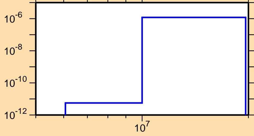
\sigma vs. E for ^{229}\text{Np}(n,2n\alpha)
