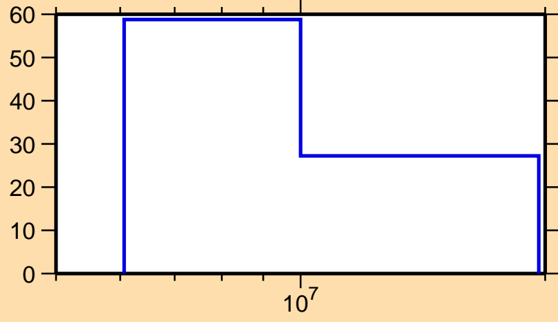
\Delta\sigma/\sigma vs. E for ^{229}\text{Np}(n,2n)
