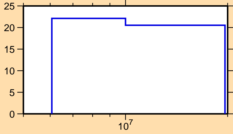
\Delta\sigma/\sigma vs. E for ^{229}\text{Np}(n,\text{nonel.})
