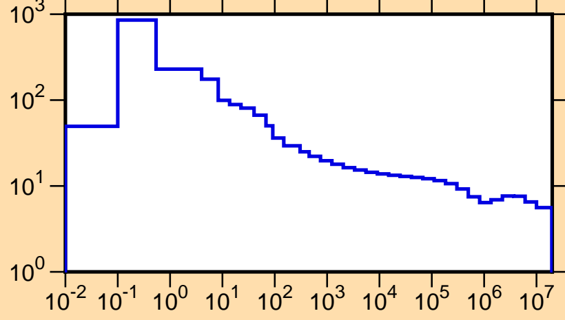
\sigma vs. E for ^{229}\text{Np}(n,\text{tot.})
