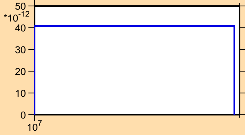
\sigma vs. E for ^{229}\text{Np}(\text{mt117})
