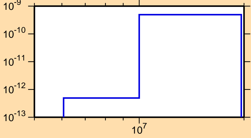
\sigma vs. E for ^{229}\text{Np}(n,p\alpha)
