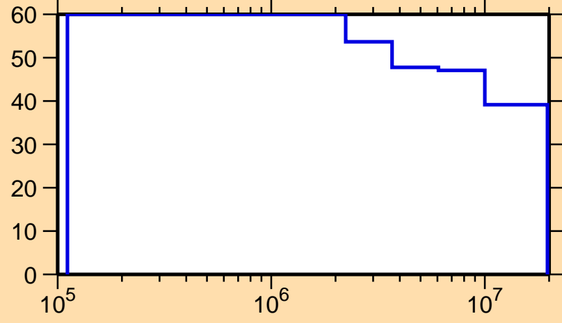
\Delta\sigma/\sigma vs. E for ^{229}\text{Np}(n,n_1)
