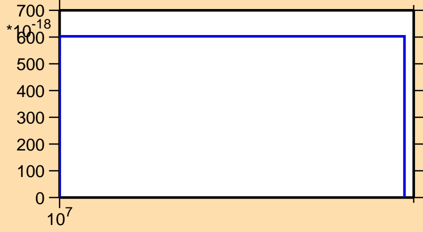
\sigma vs. E for ^{229}\text{Np} (mt 11)
