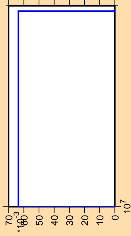
\Delta\sigma/\sigma vs. E for ^{229}\text{Np} (mt 34)
