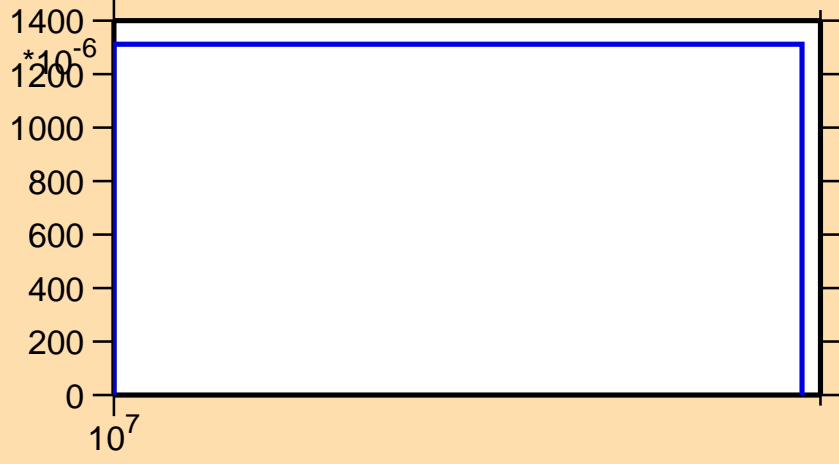
\sigma vs. E for ^{229}\text{Np}(n,3n)
