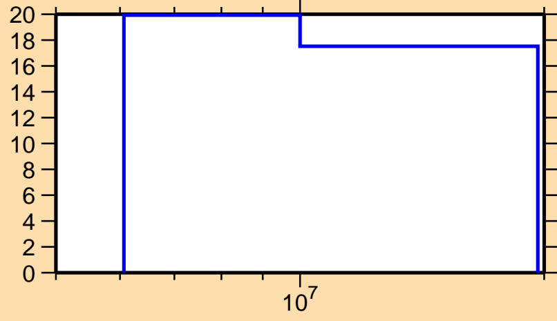
\Delta\sigma/\sigma vs. E for ^{229}\text{Np}(n,\text{el.})
