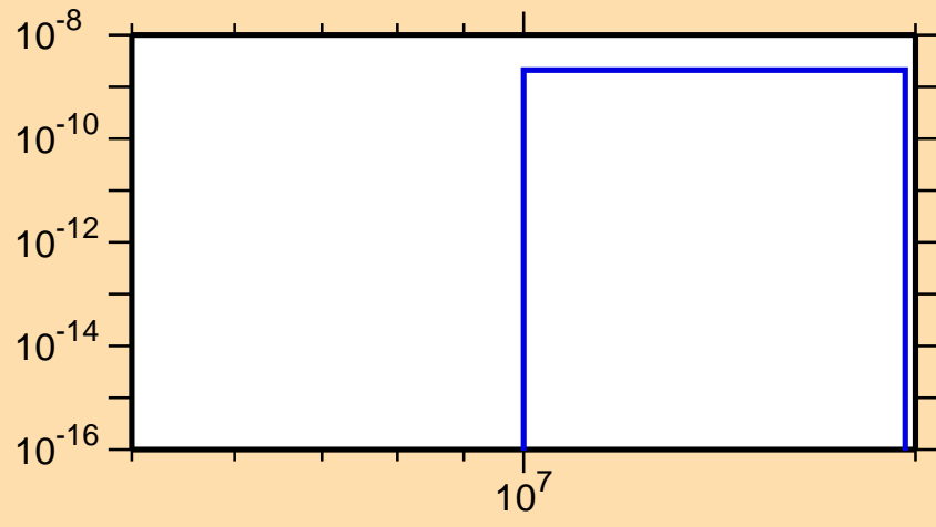
\sigma vs. E for ^{229}\text{Np}(n,\text{He3})
