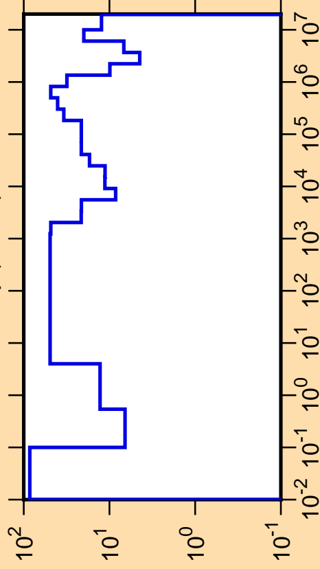
\Delta\sigma/\sigma vs. E for ^{229}\text{Np}(n,\text{tot.})
