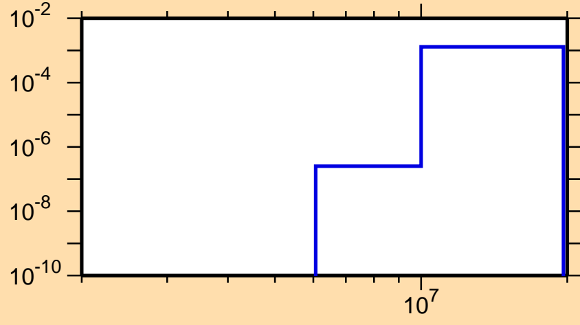
\sigma vs. E for ^{229}\text{Np}(n,d)
