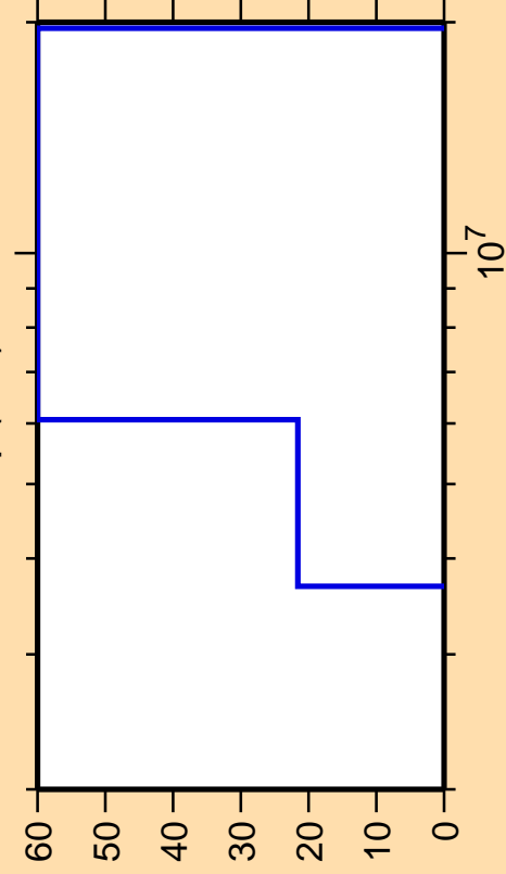
\Delta\sigma/\sigma vs. E for ^{229}\text{Np}(n,d)
