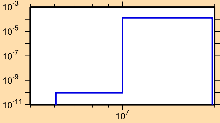
\sigma vs. E for ^{229}\text{Np}(n,t)
