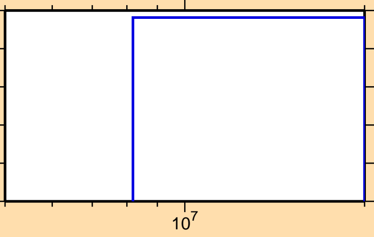
\sigma vs. E for ^{229}\text{Np}(n,2n\alpha)
