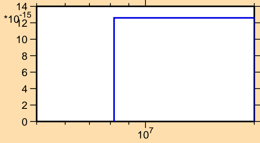
\sigma vs. E for ^{229}\text{Np}(\text{mt } 34)
