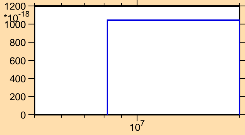
\sigma vs. E for ^{229}\text{Np}(n,\text{pd})
