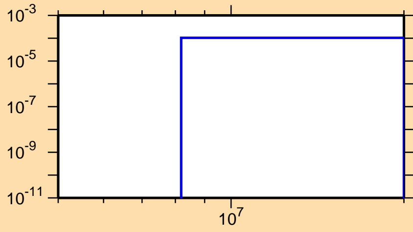
\sigma vs. E for ^{229}\text{Np}(n,t)
