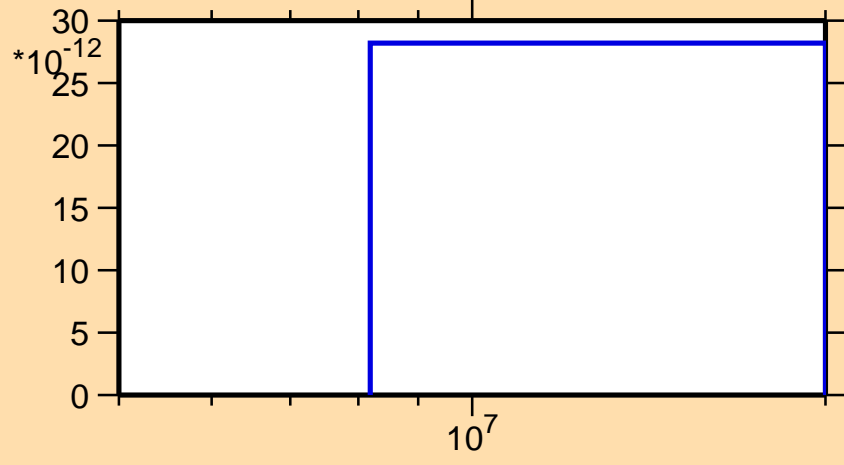
\sigma vs. E for ^{229}\text{Np}(\text{mt } 45)
