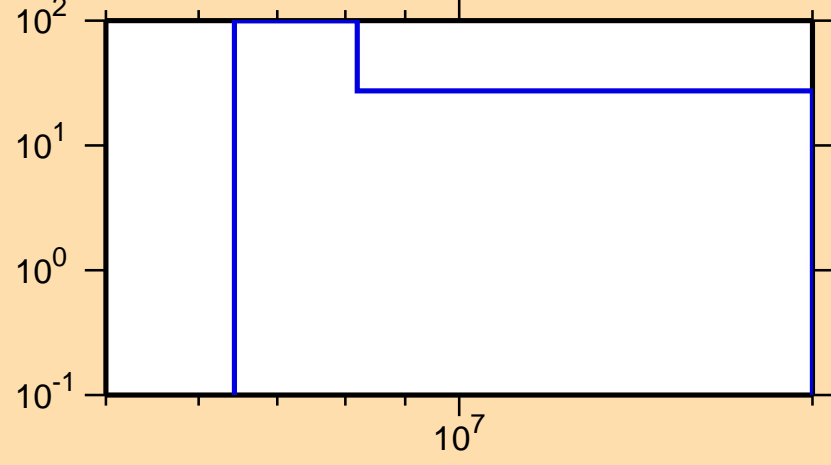
\Delta\sigma/\sigma vs. E for ^{229}\text{Np}(n,2n)
