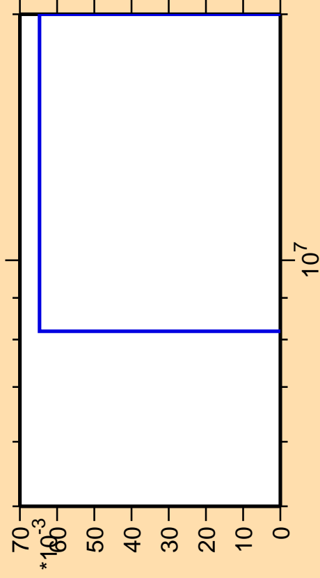
\Delta\sigma/\sigma vs. E for ^{229}\text{Np}(\text{mt } 34)
