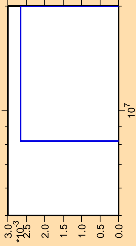
\Delta\sigma/\sigma vs. E for ^{229}\text{Np}(\text{mt } 11)
