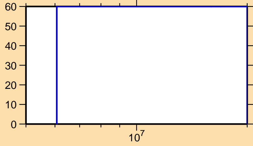
\Delta\sigma/\sigma vs. E for ^{230}\text{Np}(n,\text{inel.})
