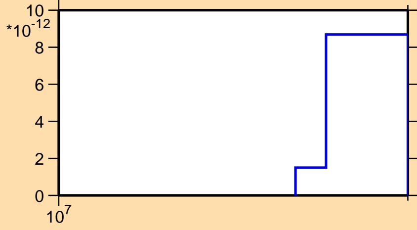
\sigma vs. E for ^{230}\text{Np} (mt 45)
