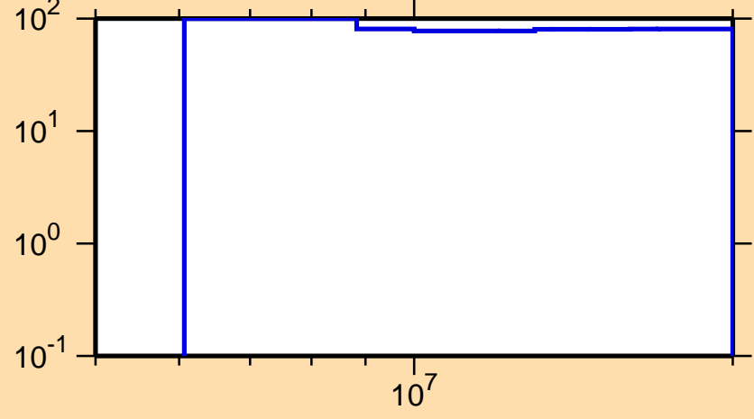
\Delta\sigma/\sigma vs. E for ^{230}\text{Np}(n,2n)
