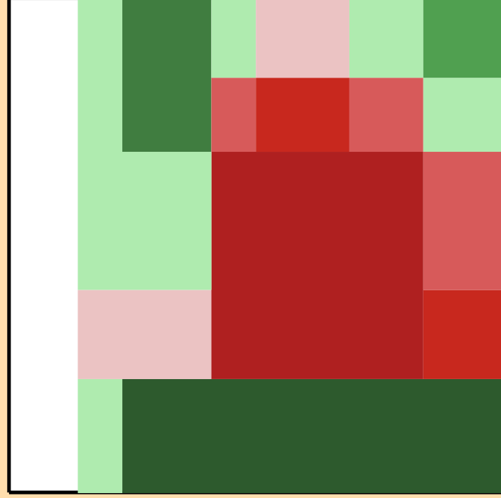
\Delta\sigma/\sigma vs. E for ^{230}\text{Np}(n,2n)
