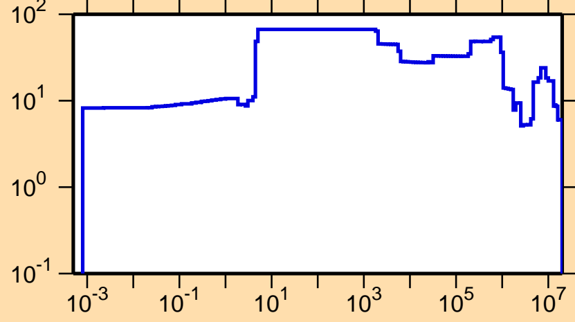
\Delta\sigma/\sigma vs. E for ^{230}\text{Np}(n,\text{tot.})
