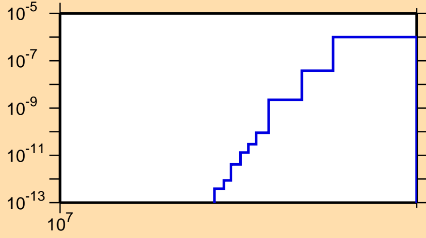
\sigma vs. E for ^{230}\text{Np}(n,nt)
