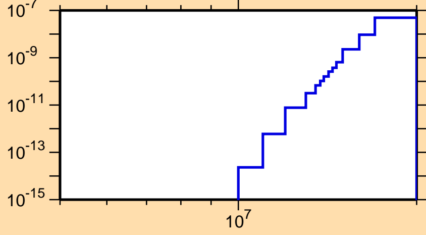
\sigma vs. E for ^{230}\text{Np}(n,\text{He3})
