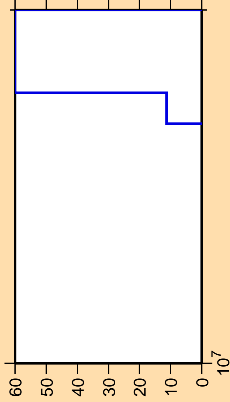
\Delta\sigma/\sigma vs. E for ^{230}\text{Np} (mt 45)
