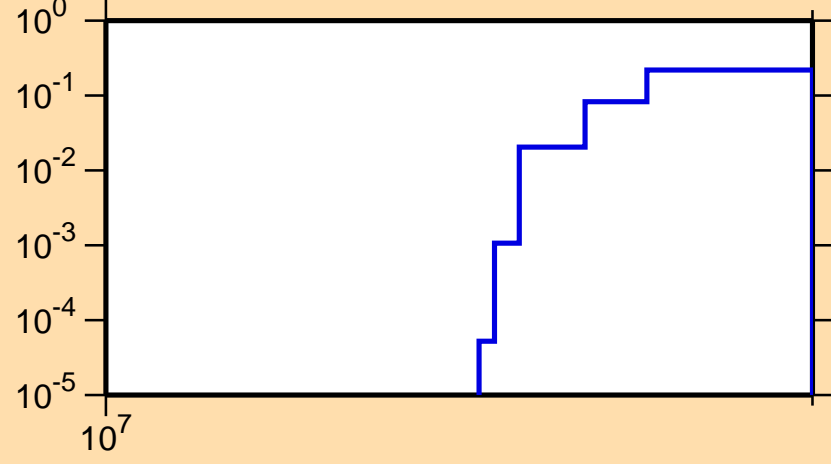
\sigma vs. E for ^{230}\text{Np}(n,3n)
