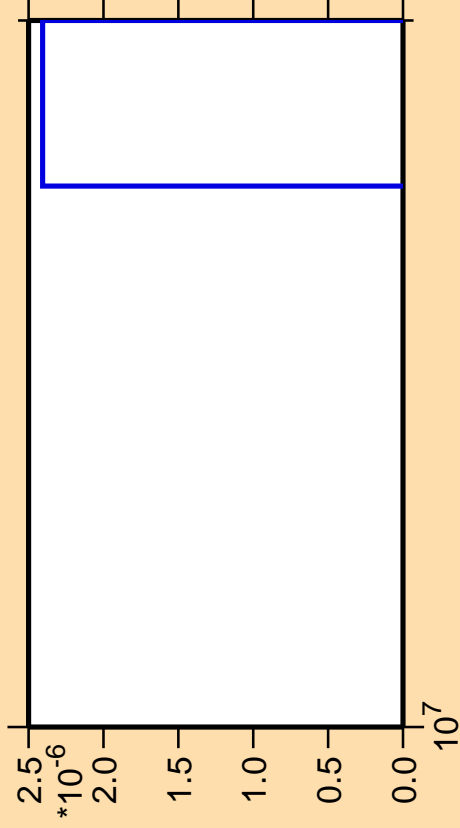
\Delta\sigma/\sigma vs. E for ^{230}\text{Np} (mt 11)
