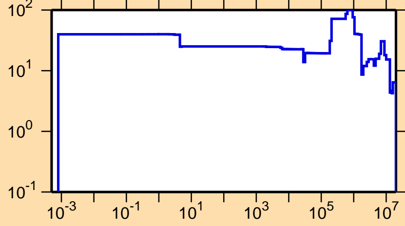
\Delta\sigma/\sigma vs. E for ^{230}\text{Np}(n,\text{el.})
