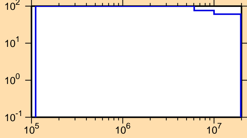
\Delta\sigma/\sigma vs. E for ^{230}\text{Np}(n,\text{inel.})
