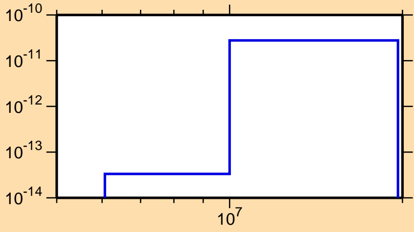
\sigma vs. E for ^{230}\text{Np}(n,p\alpha)
