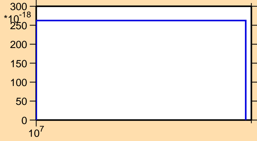
\sigma vs. E for ^{230}\text{Np} (mt 11)
