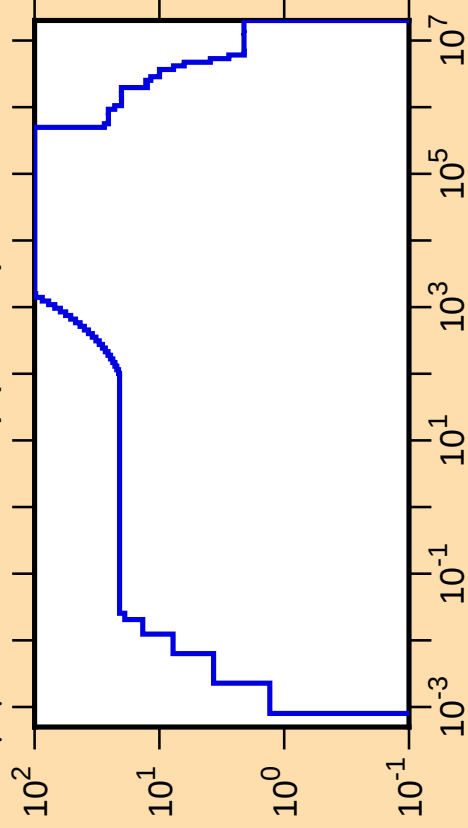
\Delta\mu/\mu vs. E for ^{231}\text{Np}(\text{mt251})
