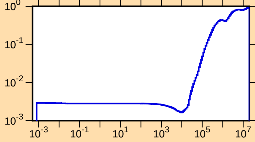
\mu vs. E for ^{231}\text{Np}(\text{mt251})
