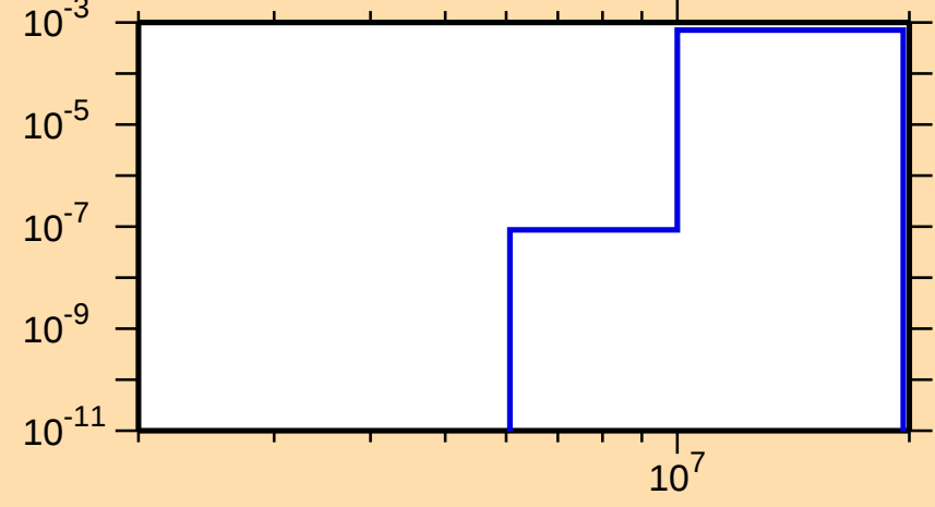
\sigma vs. E for ^{231}\text{Np}(n,d)
