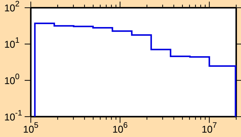
\Delta\sigma/\sigma vs. E for ^{231}\text{Np}(n,\text{nonel.})
