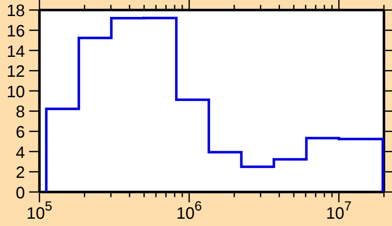
\Delta\sigma/\sigma vs. E for ^{231}\text{Np}(n,\text{tot.})
