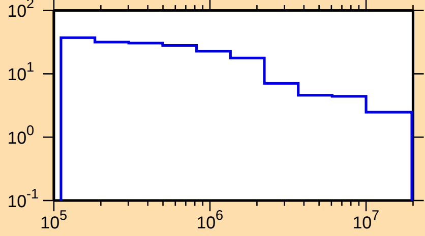
\Delta\sigma/\sigma vs. E for ^{231}\text{Np}(n,\text{nonel.})
