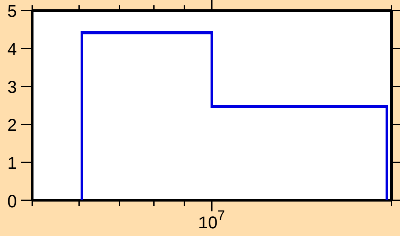
\Delta\sigma/\sigma vs. E for ^{231}\text{Np}(n,\text{nonel.})
