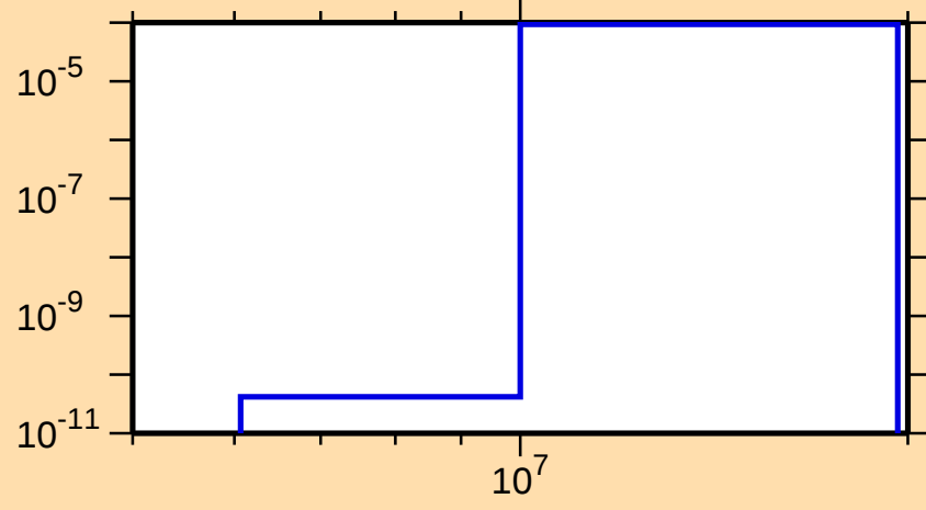
\sigma vs. E for ^{231}\text{Np}(n,t)
