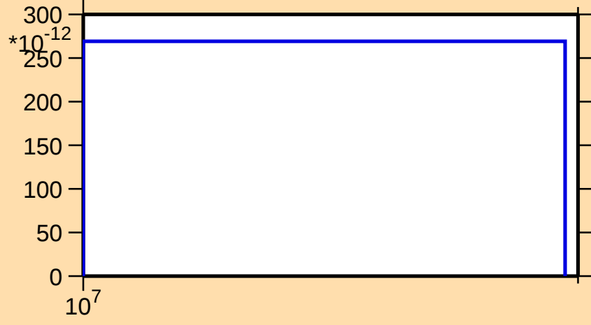
\sigma vs. E for ^{231}\text{Np}(n,\text{nd})
