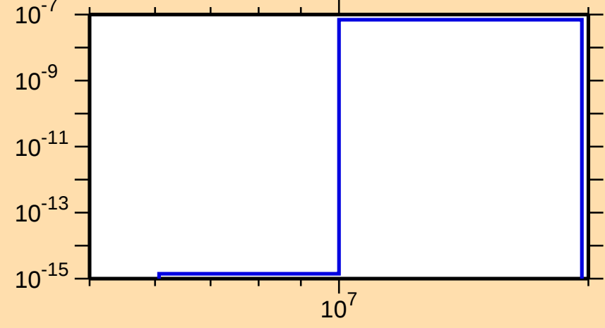
\sigma vs. E for ^{231}\text{Np}(n,2n\alpha)
