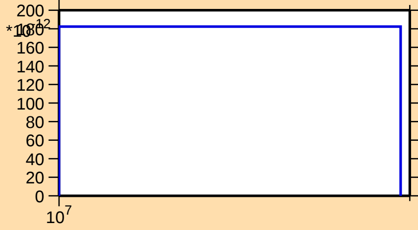
\sigma vs. E for ^{231}\text{Np}(n,\text{He3})
