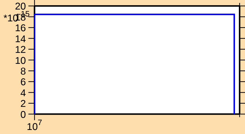
\sigma vs. E for ^{231}\text{Np} (mt 45)
