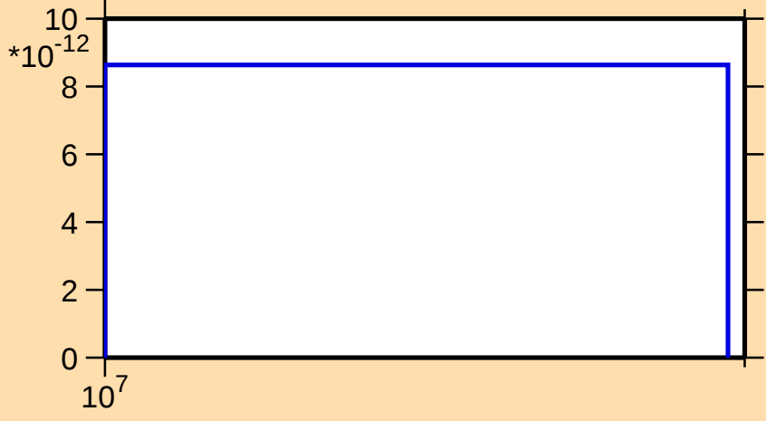
\sigma vs. E for ^{231}\text{Np}(n,p\alpha)
