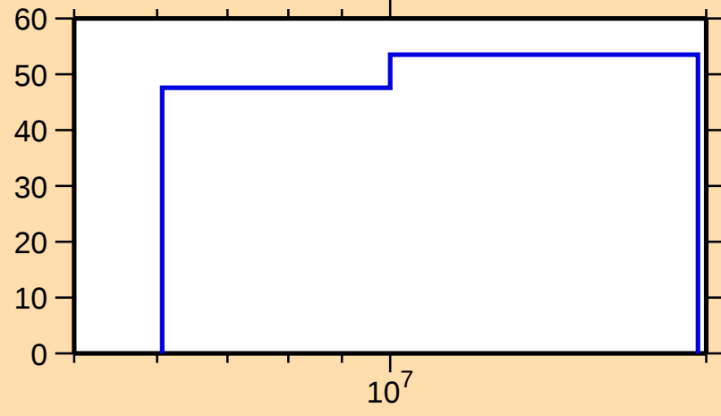
\Delta\sigma/\sigma vs. E for ^{231}\text{Np}(n,\text{inel.})
