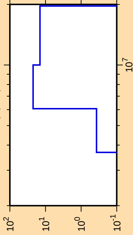
\Delta\sigma/\sigma vs. E for ^{231}\text{Np}(n,d)
