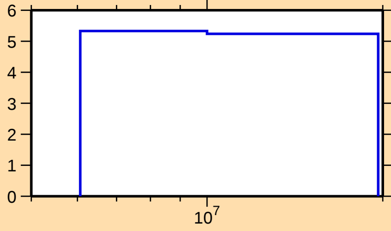
\Delta\sigma/\sigma vs. E for ^{231}\text{Np}(n,\text{tot.})
