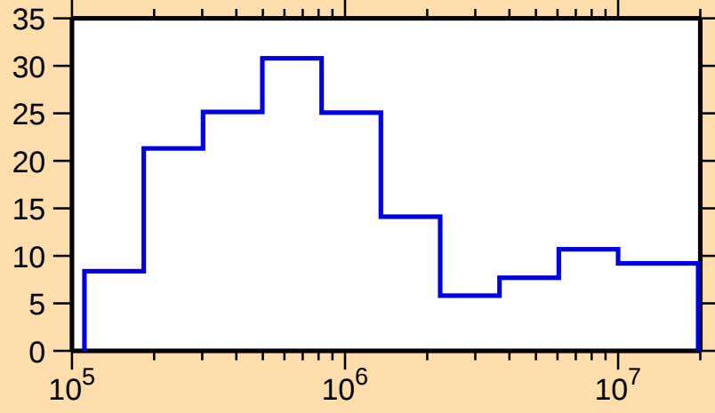
\Delta\sigma/\sigma vs. E for ^{231}\text{Np}(n,\text{el.})
