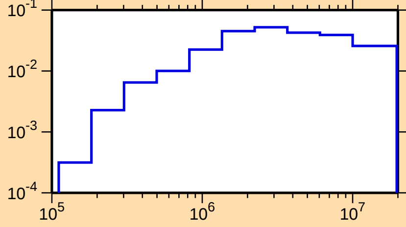
\sigma vs. E for ^{231}\text{Np}(n,\text{inel.})
