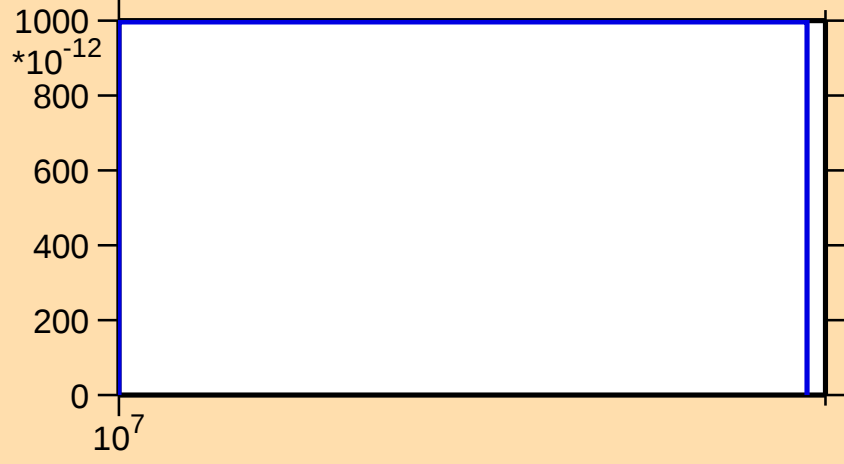
\sigma vs. E for ^{231}\text{Np}(n,2np)
