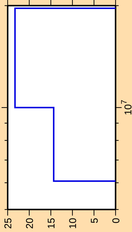
\Delta\sigma/\sigma vs. E for ^{231}\text{Np}(n,t)
