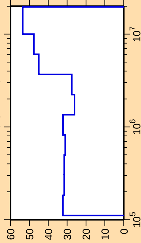
\Delta\sigma/\sigma vs. E for ^{231}\text{Np}(n,\text{inel.})
