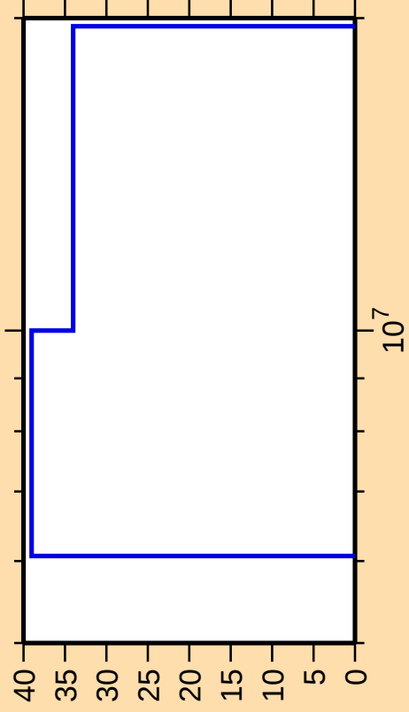
\Delta\sigma/\sigma vs. E for ^{231}\text{Np}(n,n_1)
