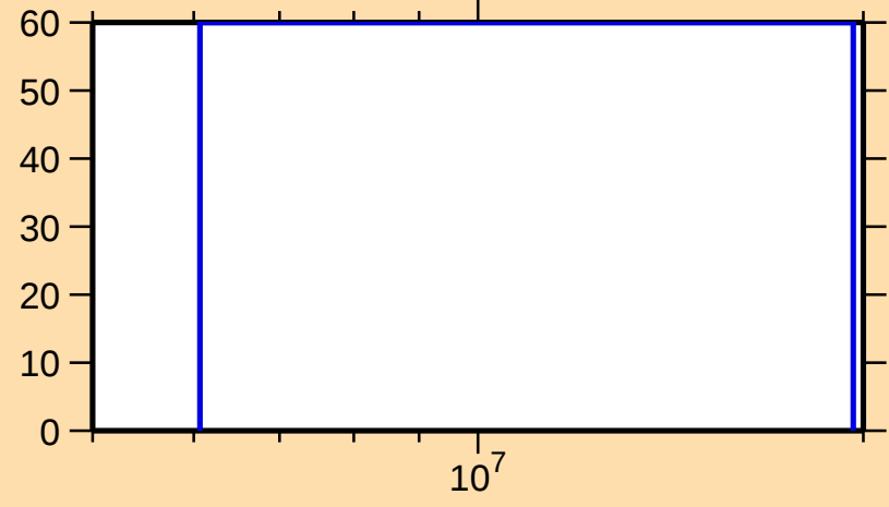
\Delta\sigma/\sigma vs. E for ^{231}\text{Np}(n,2n)
