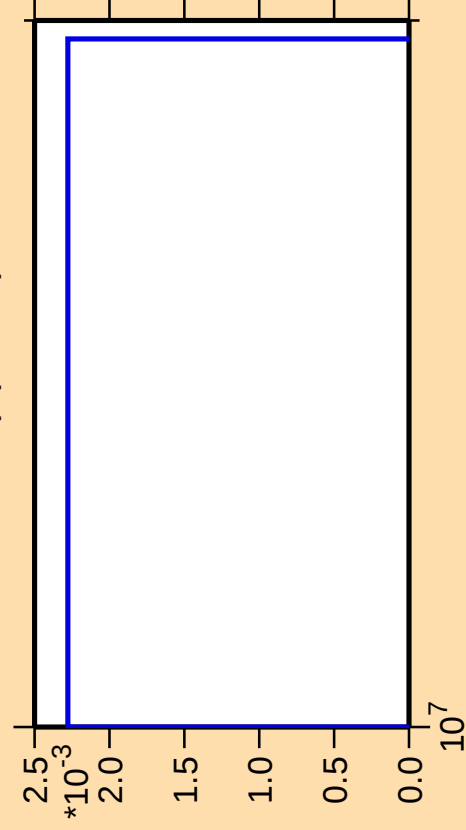
\Delta\sigma/\sigma vs. E for ^{231}\text{Np}(\text{mt 11})
