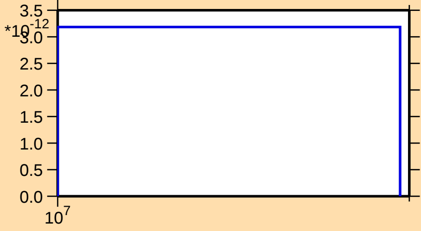
\sigma vs. E for ^{231}\text{Np}(n,3n\alpha)
