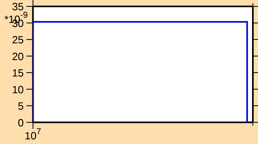
\sigma vs. E for ^{231}\text{Np}(n,nt)
