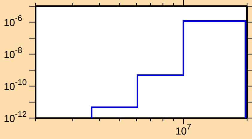
\sigma vs. E for ^{231}\text{Np}(n,\alpha)
