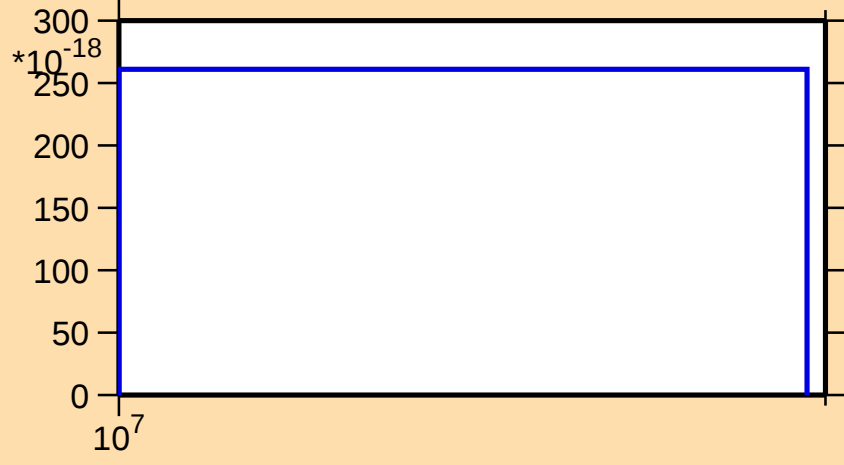
\sigma vs. E for ^{231}\text{Np}(\text{mt 11})
