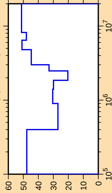
\Delta\sigma/\sigma vs. E for ^{231}\text{Np}(n,\text{ncont.})
