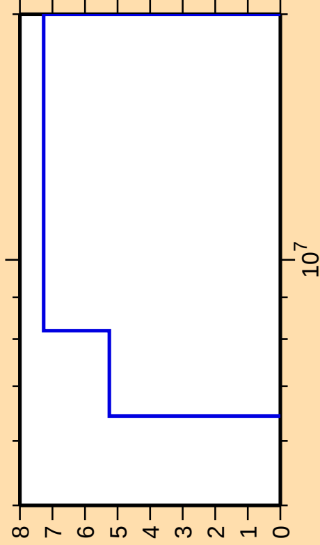
\Delta\sigma/\sigma vs. E for ^{231}\text{Np}(n,f)
