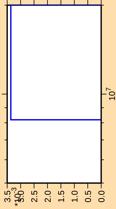
\Delta\sigma/\sigma vs. E for ^{231}\text{Np}(\text{mt 11})
