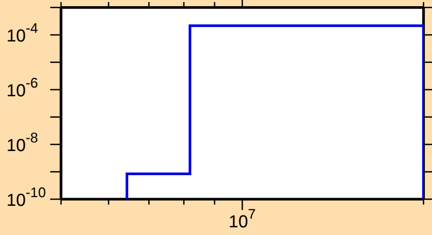
\sigma vs. E for ^{231}\text{Np}(n,np)
