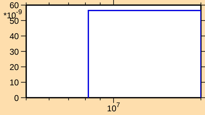
\sigma vs. E for ^{231}\text{Np}(n,2n\alpha)
