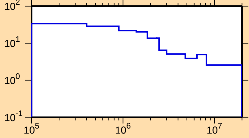
\Delta\sigma/\sigma vs. E for ^{231}\text{Np}(n,n\text{onel.})
